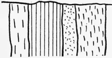
Fig. 9. Section of vertical beds. The width of outcrop is the same as the actual width of the bed.
