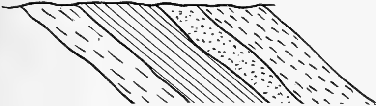
Fig. 8. Section showing outcropping beds of tilted strata.
