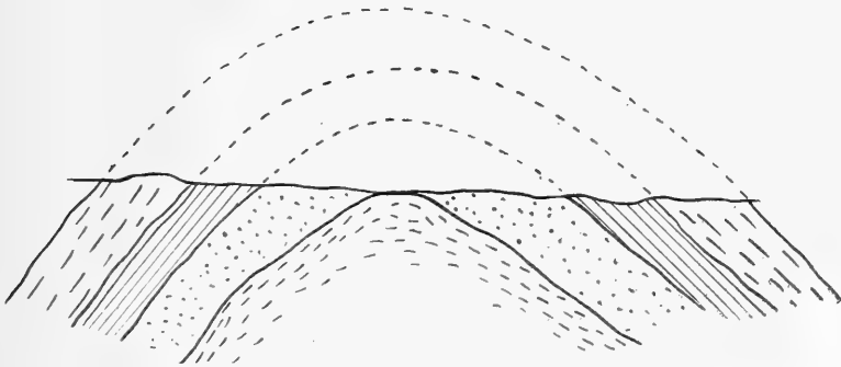
Fig. 10. Section of folded beds, with crest worn away, thus exposing the different layers.
