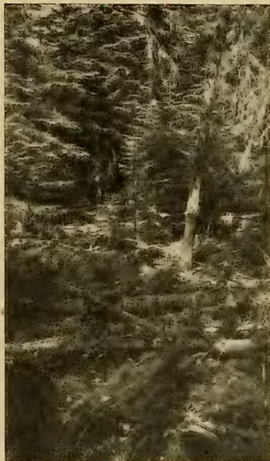
FIG. 3.—Illustrates conditions resulting from a windfall in the climax forest: fallen trunks and young balsams; Smithwick Island.
