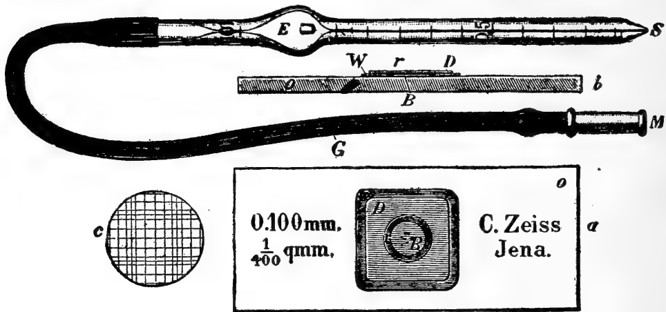
FIG. 1. The Thoma hematocytometer.
