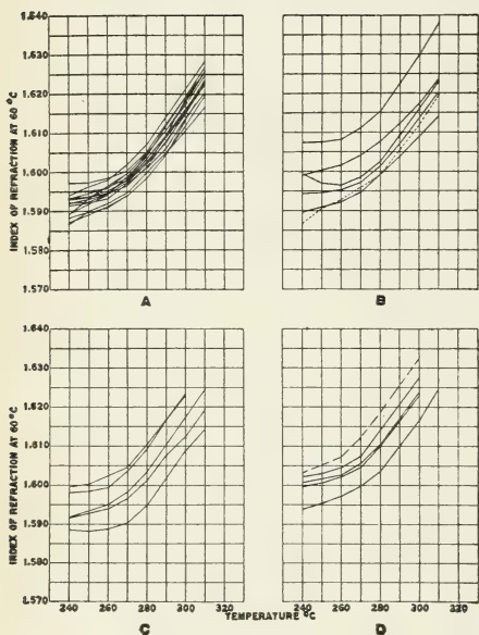
FIG. 18.—Index of refraction values of fractions of authentic coal-tar creosotes.
