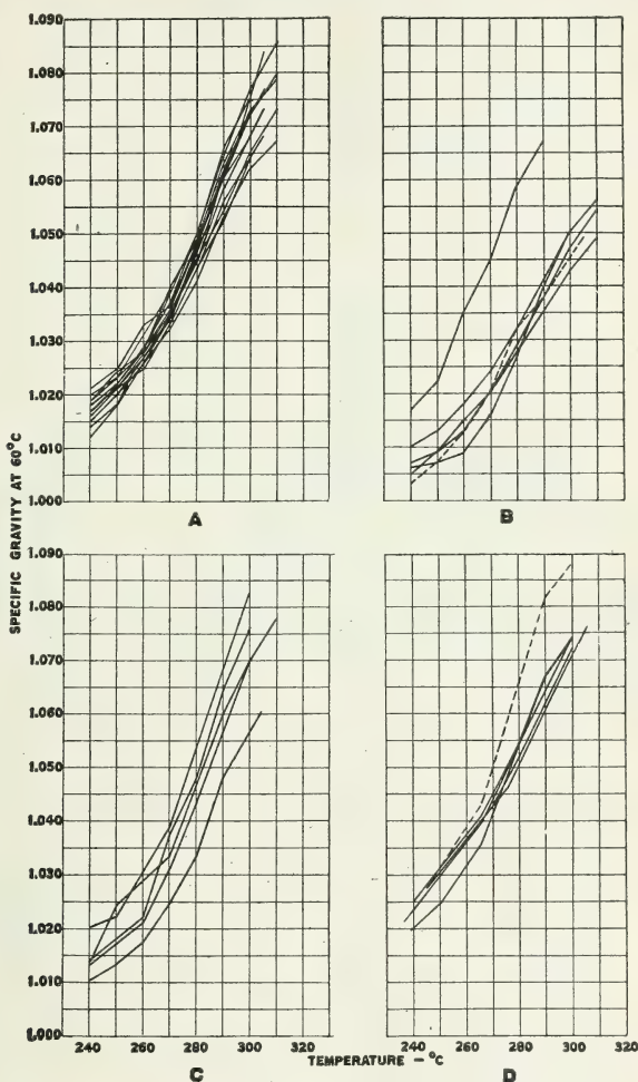
FIG. 19.—Specific gravities of fractions of authentic coal-tar creosotes.
