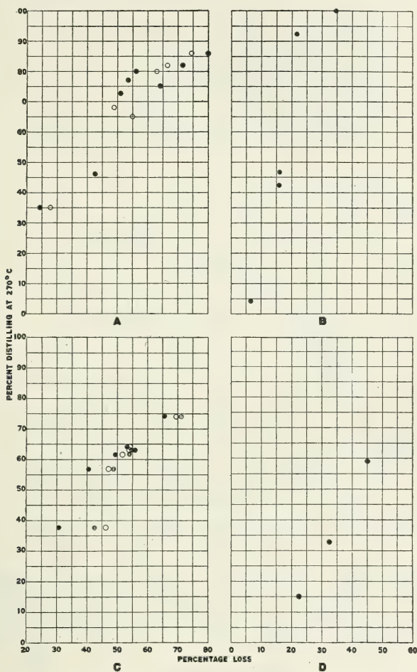
FIG. 31.—Relation between the loss by evaporation and the per cent of the oil volatile below 270° C.
