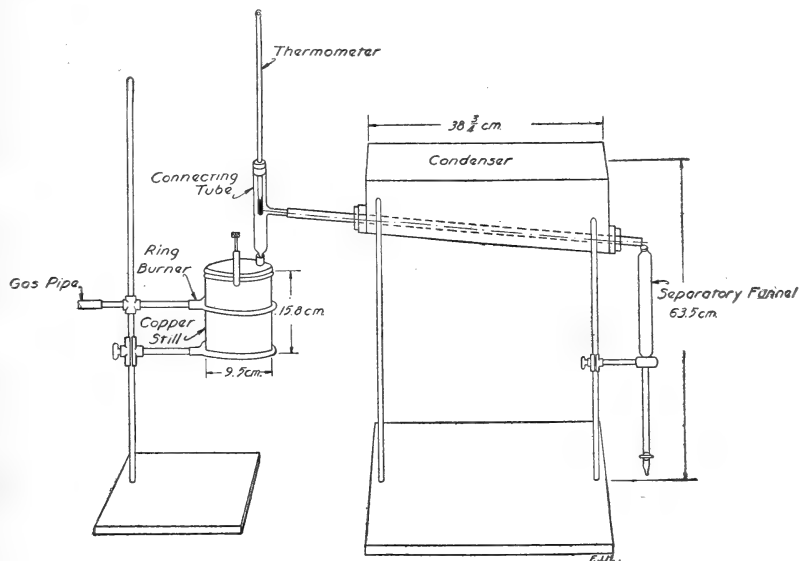
FIG. 46.—Apparatus for determining moisture content of cerosote oil.
