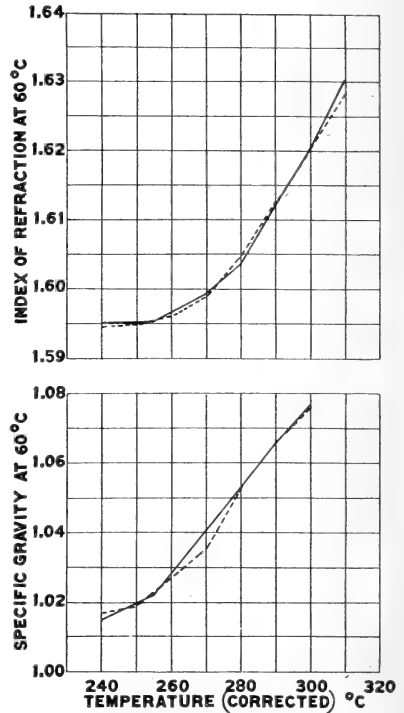
FIG. 16.—Physical constants of two coal-tar creosotes produced from tar No. 2.
