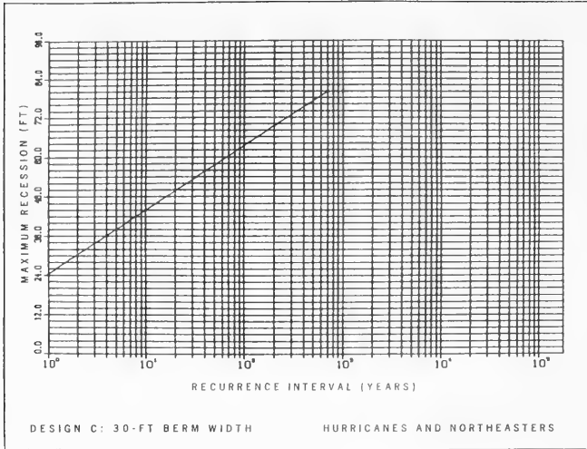
Figure 48. Maximum recession-recurrence design curve for combined hurricanes and northeasters for Design C: 30-ft berm width
