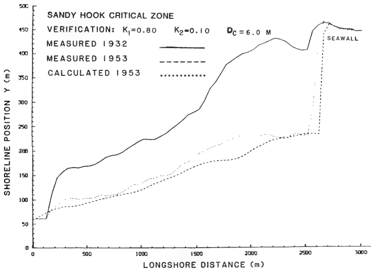
Figure 19. Results of verification 1932-1953 (maximum constant depth of closure)
