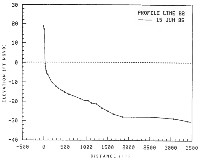
Figure 28. Profile 82
