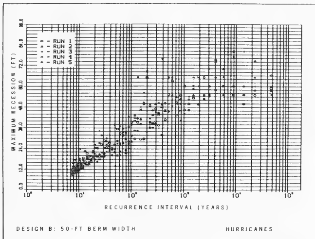
Figure 43. Hurricane recession-recurrence plot for Design B: 50-ft berm width
