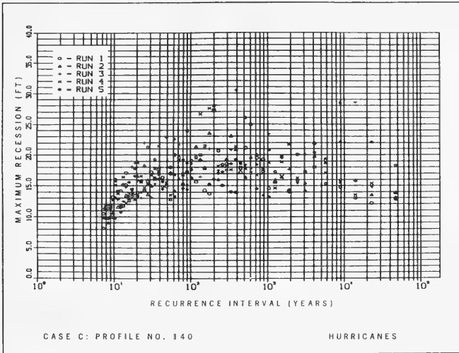
Figure 34. Hurricane recession-recurrence plot for Profile 140
