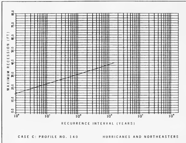
Figure 36. Maximum recession-recurrence design curve for combined hurricanes and northeasters for Profile 140
