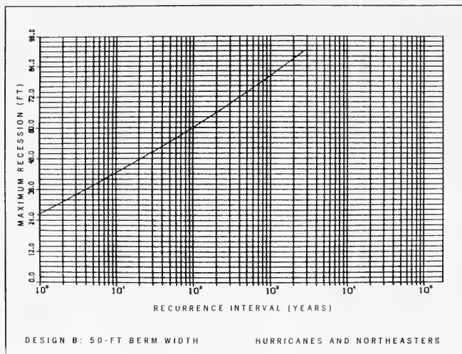
Figure 45. Maximum recession-recurrence design curve for combined hurricanes and northeasters for Design B: 50-ft berm width
