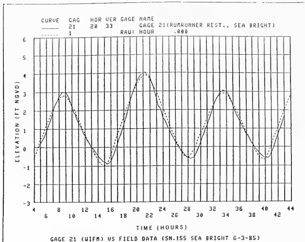
Figure 60. Tide verification data - Rumrunner Restaurant, Sea Bright (TG3)
