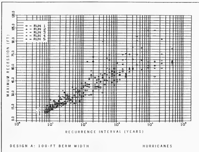
Figure 40. Hurricane recession-recurrence plot for Design A: 100-ft berm width
