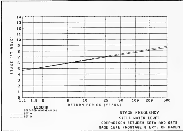
Figure 68. Variability in stage frequency for the two northeaster data sets at gage 12
