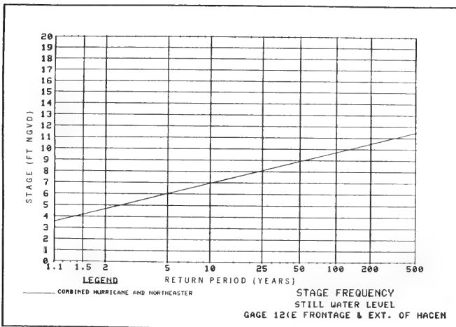
Figure 70. Stage frequency curve for the combined hurricane- and northeaster-induced water level at gage 12
