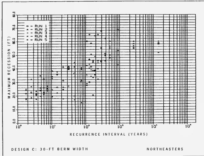
Figure 47. Northeastern recession-recurrence plot for Design C: 30-ft berm width
