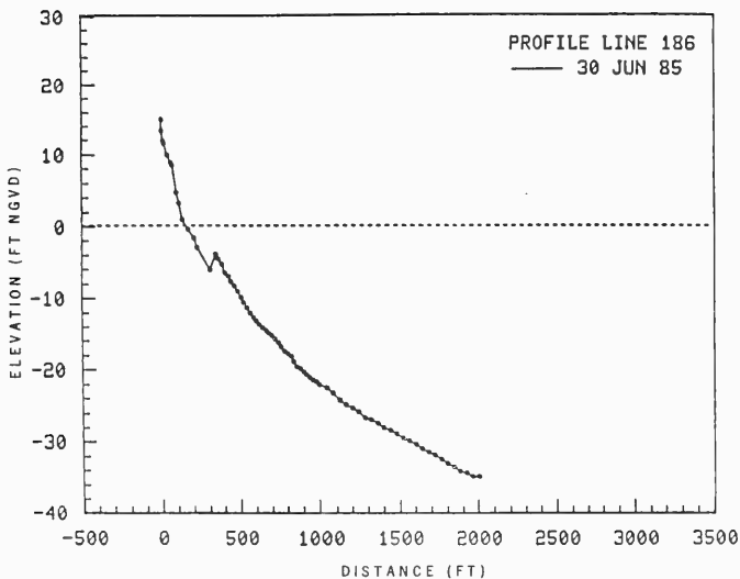
Figure 30. Profile 186
