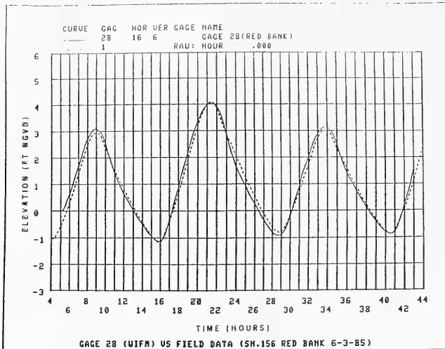
Figure 59. Tide verification data - Red Bank (TG2)
