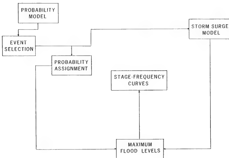
Figure 49. Flow chart of project technique
