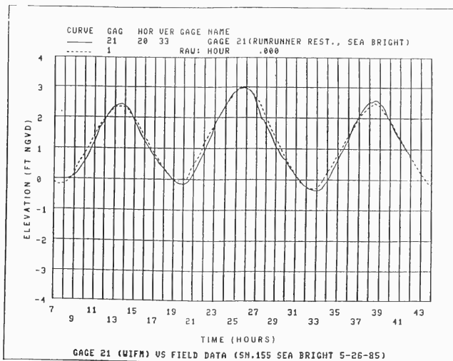
Figure 57. Tide calibration data - Rumrunner Restaurant, Sea Bright (TG3)
