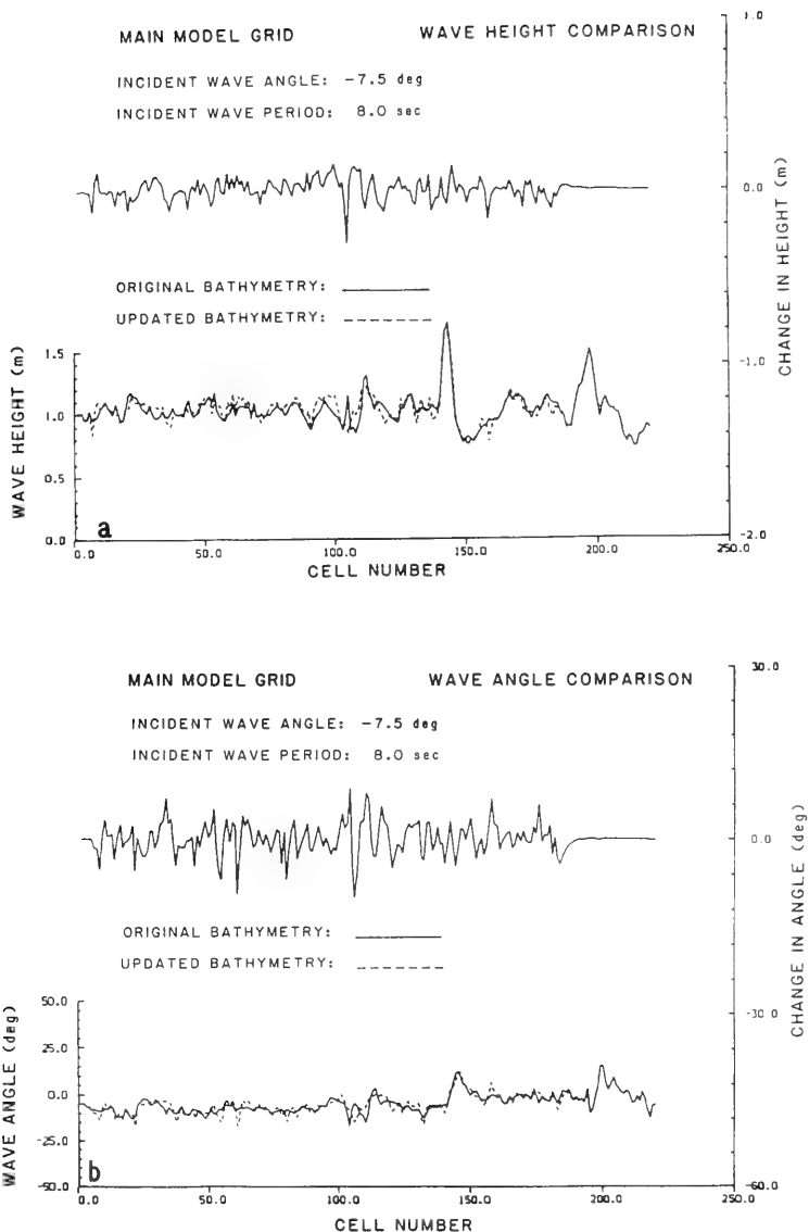
Figure 11. Comparison of calculated (a) wave height and (b) wave direction at the nominal 3-m depth alongshore for original bathymetry and bathymetry updated with 1985 profile surveys
