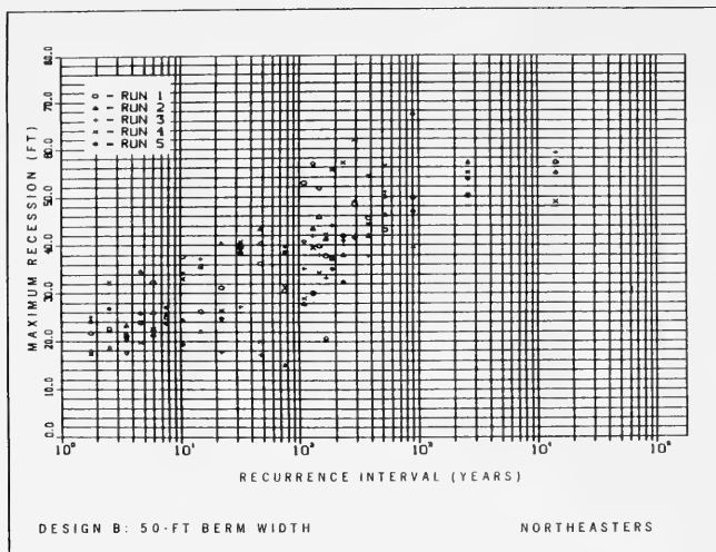
Figure 44. Northeast recession-recurrence plot for Design B: 50-ft berm width
