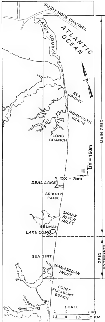
Figure 9. Grid used in the nearshore refraction calculation
