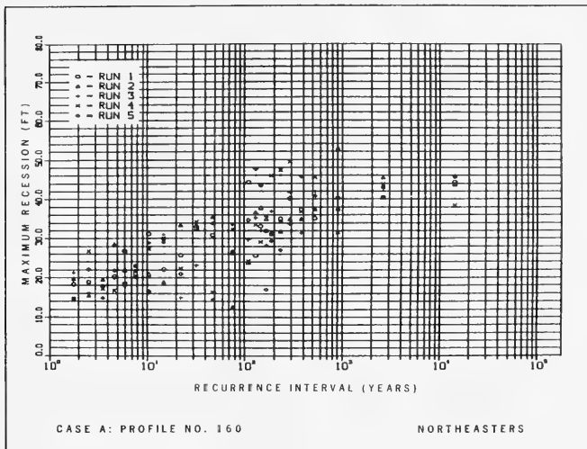
Figure 32. Northeastern recession-recurrence plot for Profile 160
