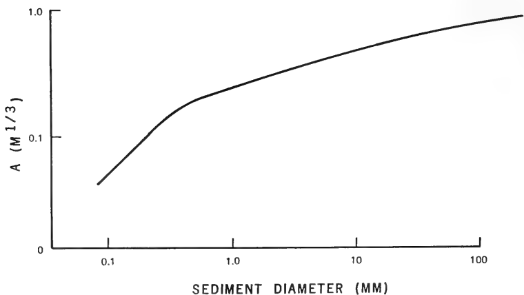
Figure 22. Shape parameter, A , versus sediment diameter (after Moore 1982)
