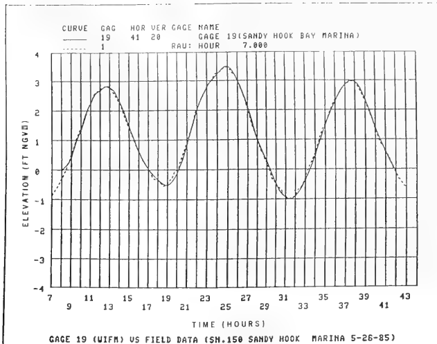
Figure 55. Tide calibration data - Sandy Hook Marina (TG1)
