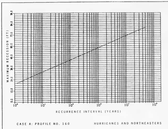
Figure 33. Maximum recession-recurrence design curve for combined hurricanes and northeasters for Profile 160
