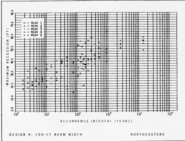
Figure 41. Northeast recession-recurrence plot for Design A: 100-ft berm width
