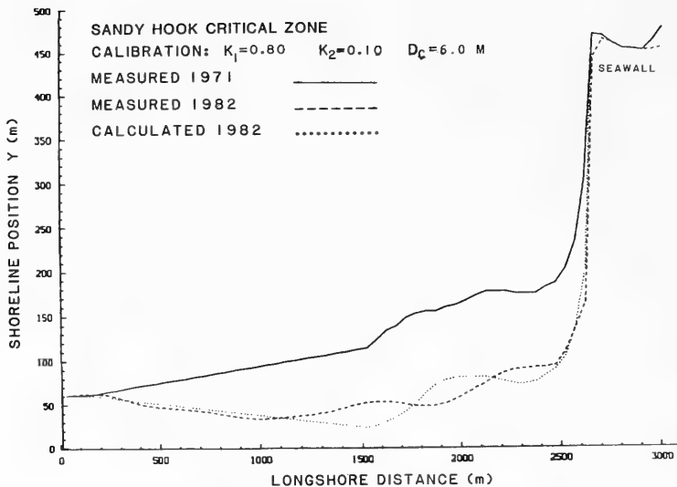
Figure 17. Results of calibration 1971-1982 (maximum constant depth of closure)
