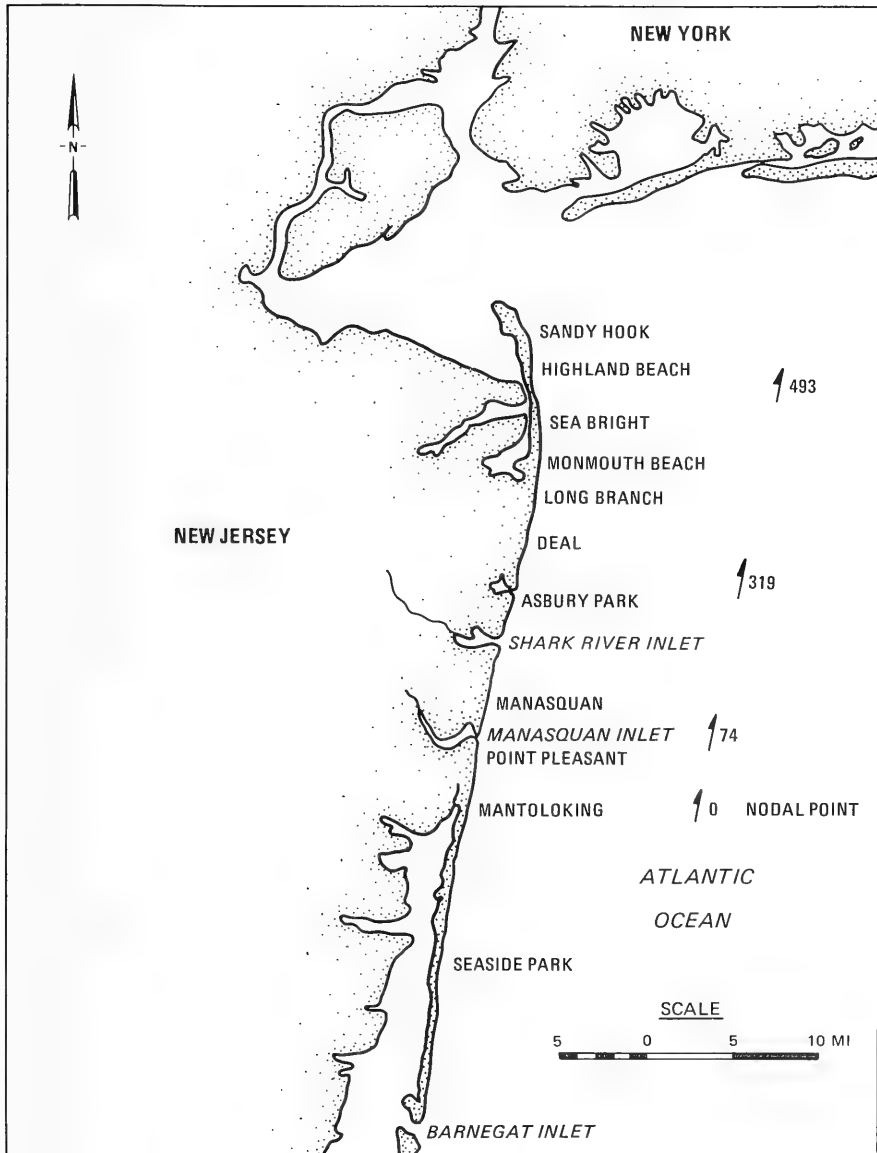
Figure 6. Historical longshore sediment transport rates (thousands of cubic yards/year) (after Caldwell 1966)
