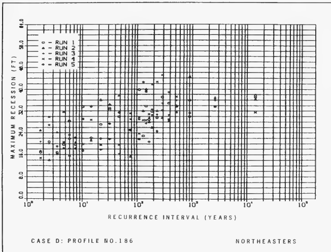
Figure 38. Northeasters recession-recurrence plot for Profile 186
