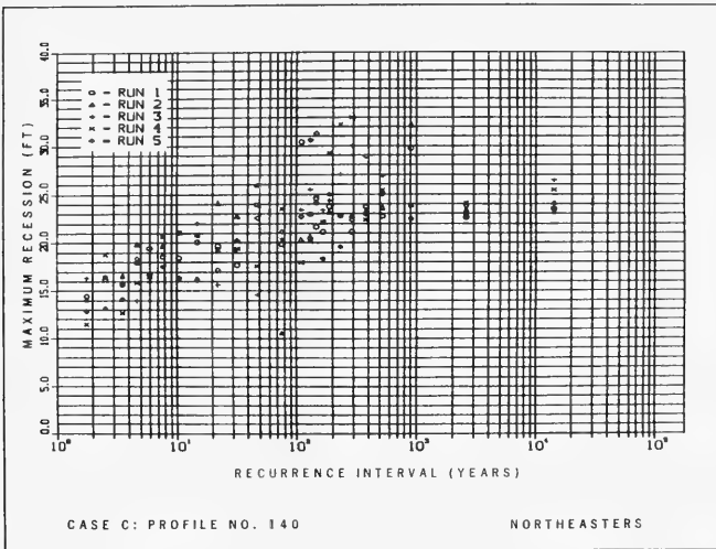
Figure 35. Northeastern recession-recurrence plot for Profile 140
