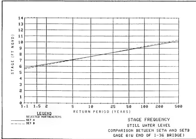
Figure 66. Variability in stage frequency for the two northeaster data sets at gage 6
