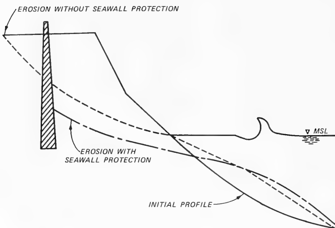
Figure 23. Conceptual seawall effects
