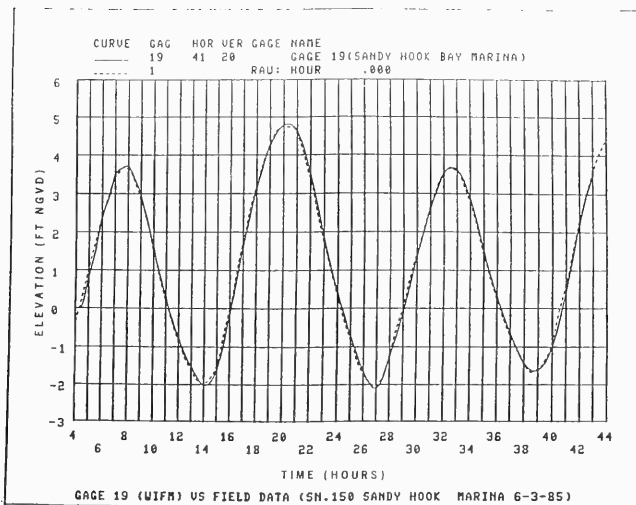
Figure 58. Tide verification data - Sandy Hook Marina (TG1)
