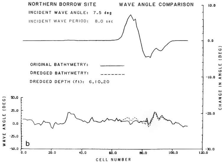
Figure 14. Change in wave properties at the nominal 3-m depth for waves refracting over the northern borrow site: (a) change in wave height, (b) change in wave direction
