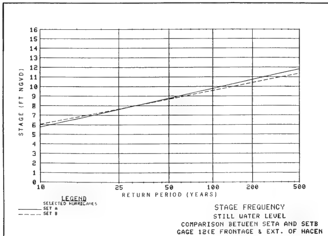
Figure 67. Variability in stage frequency for the two hurricane data sets at gage 12
