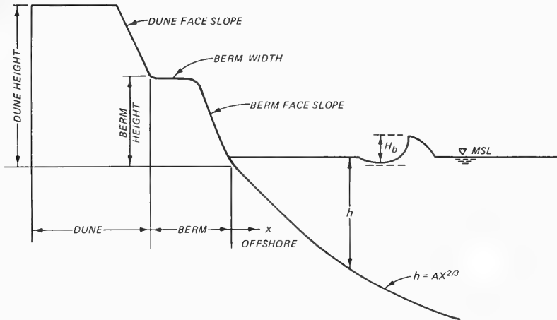
Figure 21. Schematized model area
