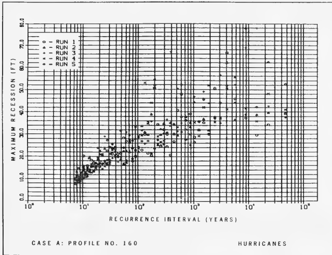
Figure 31. Hurricane recession-recurrence plot for Profile 160
