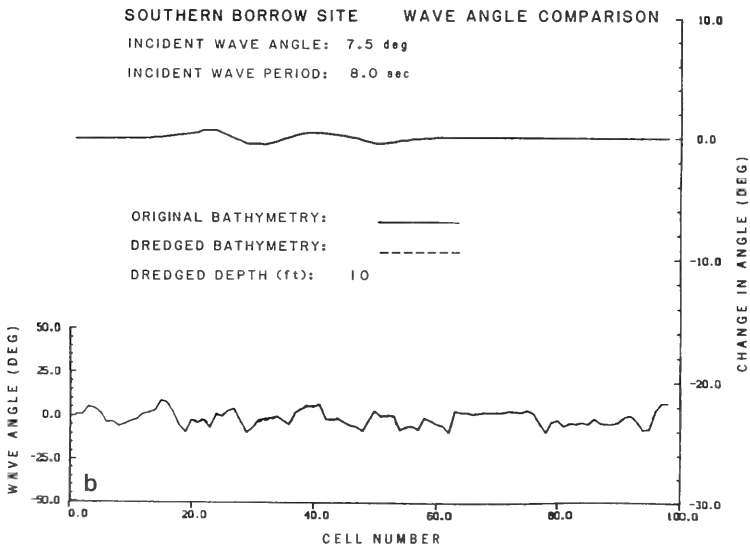
Figure 15. Change in wave properties at the nominal 3-m depth for waves refracting over the southern borrow site: (a) change in wave height, (b) change in wave direction
