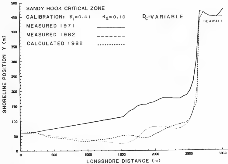
Figure 16. Results of calibration 1971-1982 (variable depth of closure)
