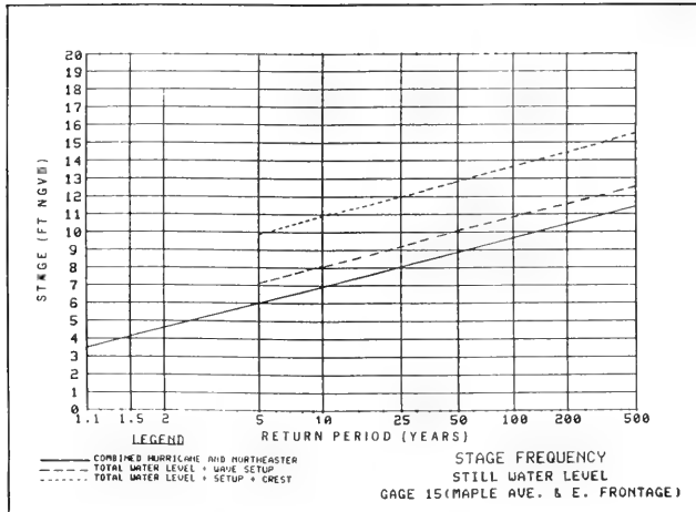
Figure 71. Estimation of maximum wave effects in the upper Navesink basin (gage 15)
