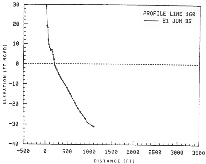
Figure 27. Profile 160
