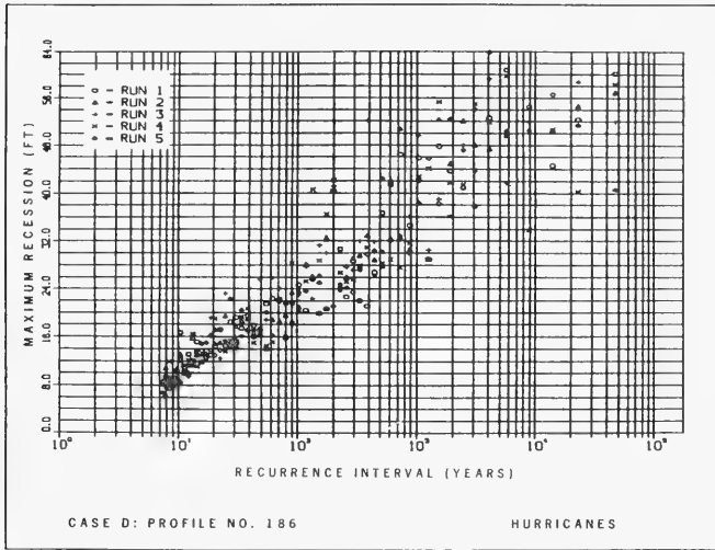
Figure 37. Hurricane recession-recurrence plot for Profile 186
