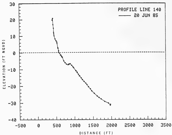
Figure 29. Profile 140
