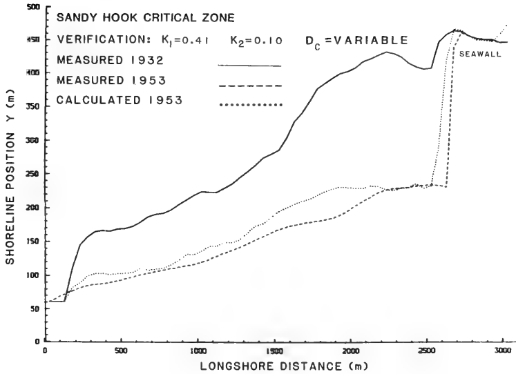
Figure 18. Results of verification 1932-1953 (variable depth of closure)
