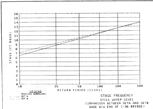
Figure 65. Variability in stage frequency for the two hurricane data sets at gage 6
