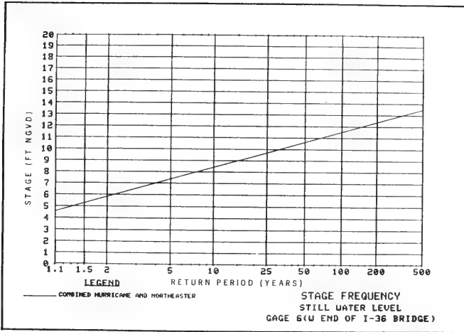
Figure 69. Stage frequency for the combined hurricane- and northeaster-induced water level at gage 6
