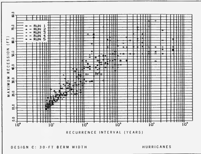
Figure 46. Hurricane recession-recurrence plot for Design C: 30-ft berm width
