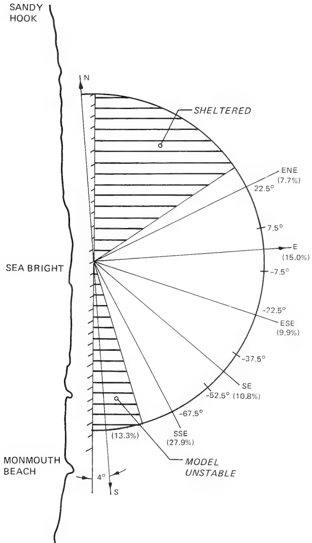
Figure 8. Wave angle bands defined by WIS relative to the shoreline trend along Sea Bright to Ocean Township
