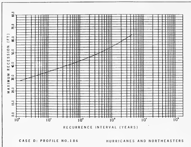
Figure 39. Maximum recession-recurrence design curve for combined hurricanes and northeasters for Profile 186
