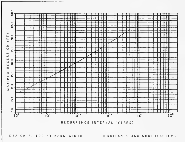
Figure 42. Maximum recession-recurrence design curve for combined hurricanes and northeasters for Design A: 100-ft berm width
