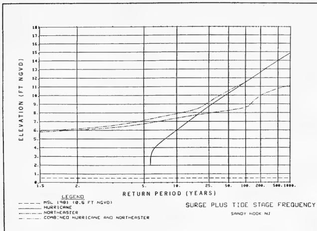
Figure 50. Still-water level stage-frequency curves - Sandy Hook, New Jersey
