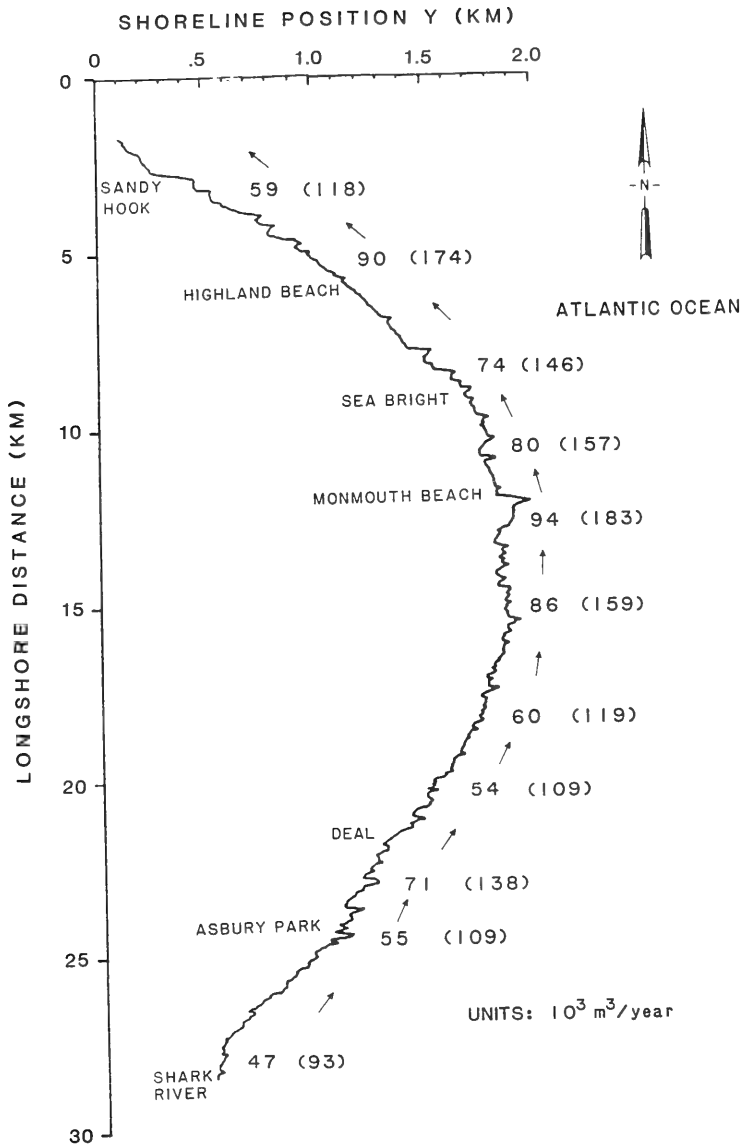
Figure 20. Calculated transport rate capacities using a variable and a constant maximum (in parentheses) depth of closure
