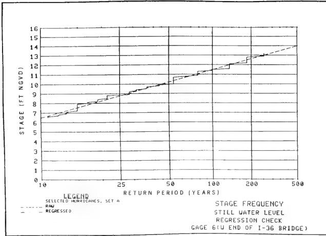
Figure 64. Example of raw and regressed stage-frequency curves
