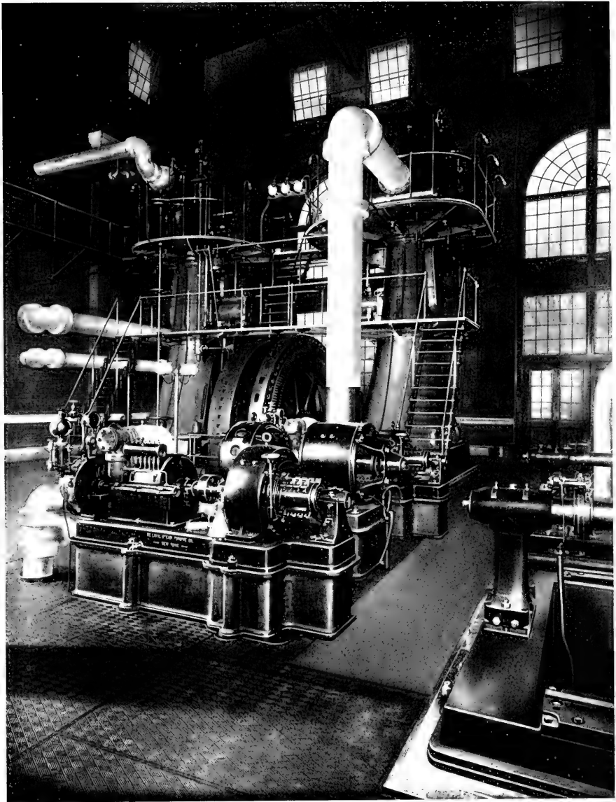
FIG. 1. THE ENGINES IN THE POWER HOUSE
