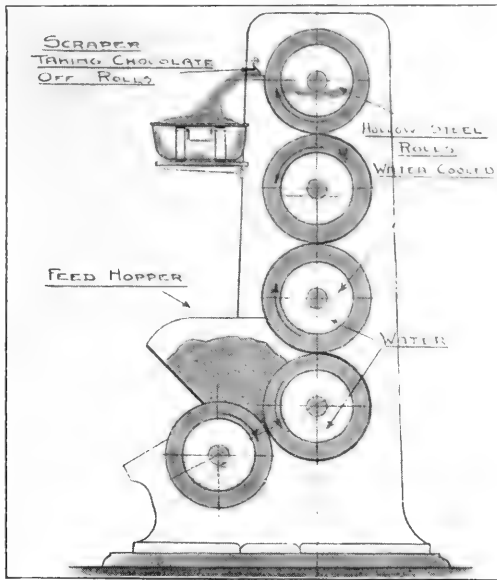
SECTION THROUGH CHOCOLATE GRINDING ROLLS.
