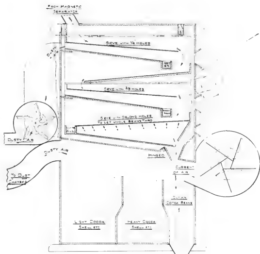
DIAGRAM OF CACAO BEAN CLEANING MACHINE.
