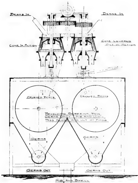
SECTION THROUGH KIBBLING CONES AND GERM SCREENS.
