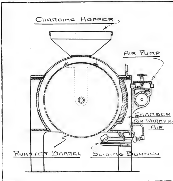
SECTION THROUGH GAS HEATED CACAO ROASTER.
