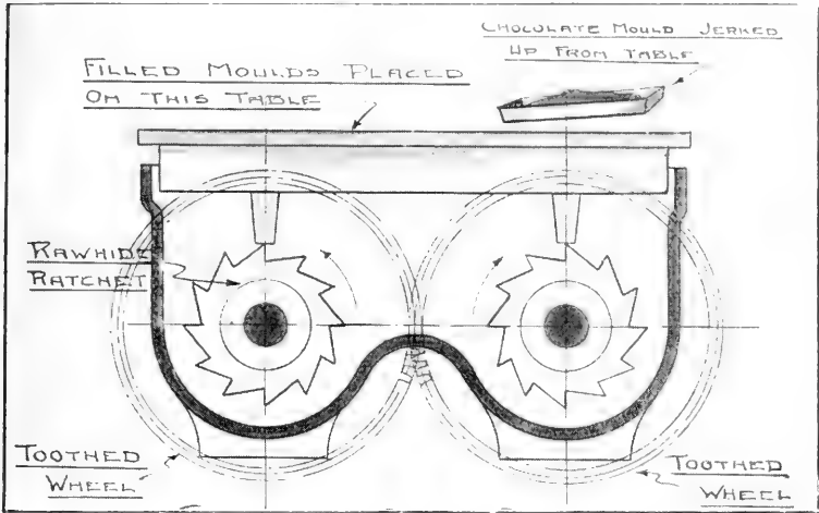
CHOCOLATE SHAKING TABLE.
