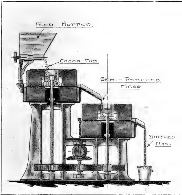
SECTION THROUGH GRINDING STONES.
