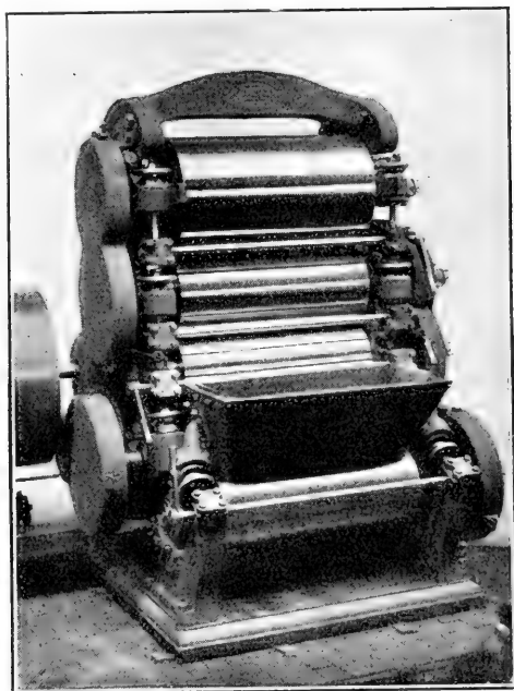
CHOCOLATE REFINING MACHINE.
