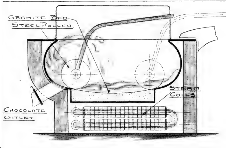
SECTION THROUGH “ CONCHE ” MACHINE.
