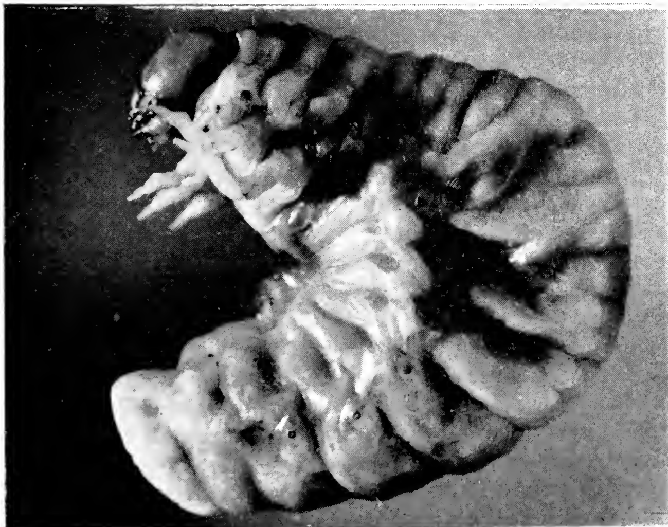
Figure 2. Third-stage larva.
