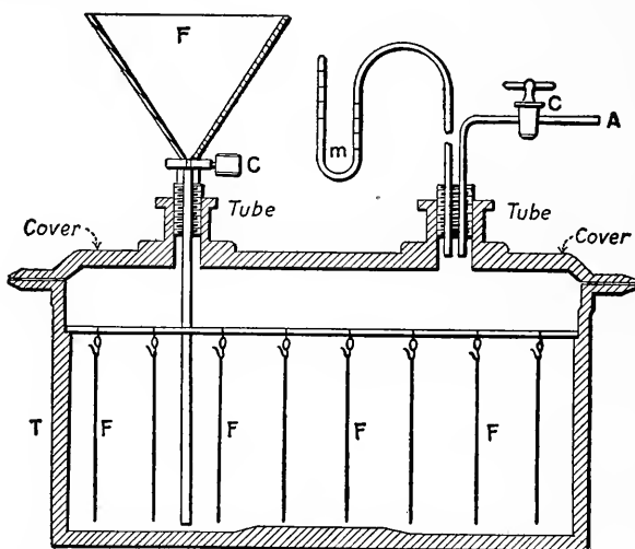
FIG. 15. Trough for the preparation of ultrafilters. (H. Bechhold.)
