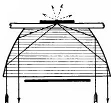
FIG. 35. Abbe condenser with central opacity.
