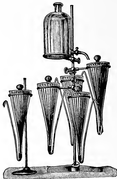
FIG. 14. Dialyzing filter. (L. Morochowetz.)
