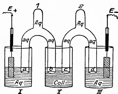
FIG. 26a. Simple apparatus for electric migration.
