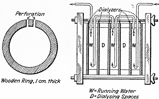
FIG. 13a. Continuous dialyzing apparatus of E. Jordiss. Reproduced from Zeitschrift für Electrochemie , p. 677, Vol. VIII, 1902.
