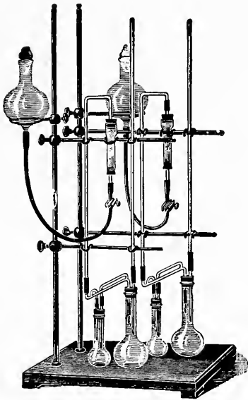
FIG. 23. Apparatus for adsorption analysis. (H. Wislicenus.)
