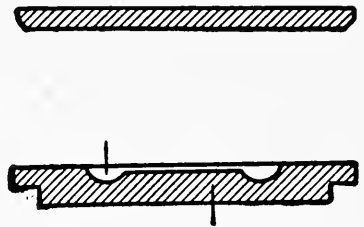
FIG. 31. Quartz chamber for the cardioid ultramicroscope.
