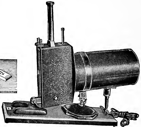
FIG. 28a. Kober Nephelometer.
