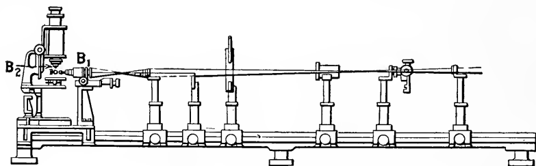
FIG. 31a. Slit-ultramicroscope.
