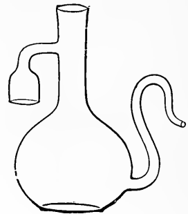
FIG. 33. Flasks for storing ultrawater. (A. Haak.)
