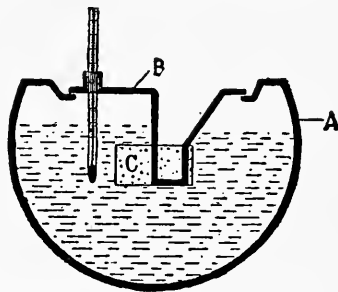
FIG. 28b. Fluid Interferometer.
