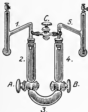
FIG. 28. Migration apparatus with non-polarizable electrodes. (L. Michaelis.)
