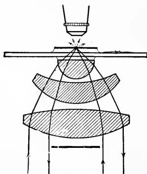
FIG. 36. Paraboloid condenser for the dark-field illumination of organisms. (From H. Siedentopf.)
