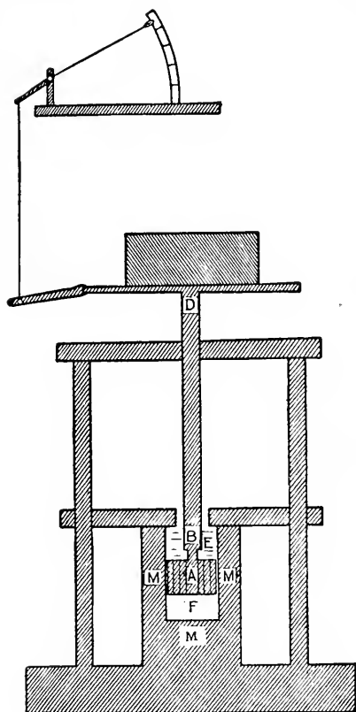
FIG. 25. J. Reinke's apparatus for measuring swelling pressure.
