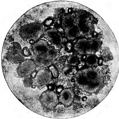
FIG. 53. Oil-droplets super-saturated with cholesterol. Crystalline separation of cholesterol may be recognized in several droplets.
