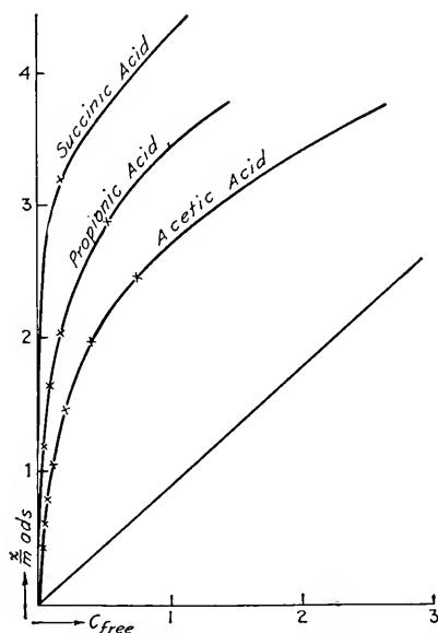
FIG. 3. Adsorption of fatty acids by charcoal. (After H. Freundlich.)
