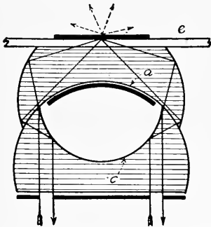
FIG. 30. Course of the light rays through the cardioid condenser. (H. Siedentopf.)
