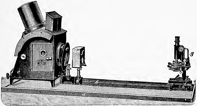
FIG. 29. Illumination of the cardioid ultramicroscope.
