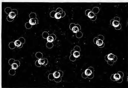
FIG. 5. Brownian movement of milk globules. (From O. Lehman.)
