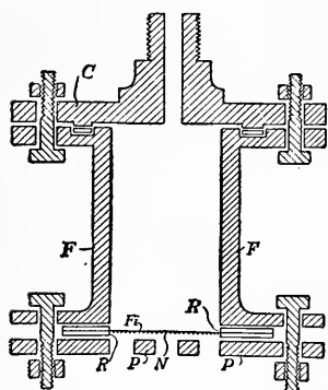
FIG. 17. Ultrafilter for high pressures.
