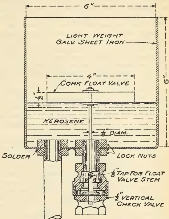
FIG. 11.—Diagram showing the construction of a float valve for the regulation of the level of kerosene in burners
