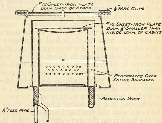
FIG. 1.—Diagram showing the method of modifying the burner of a kerosene stove with two iron plates in order to make stove gas for coloring citrus fruit
