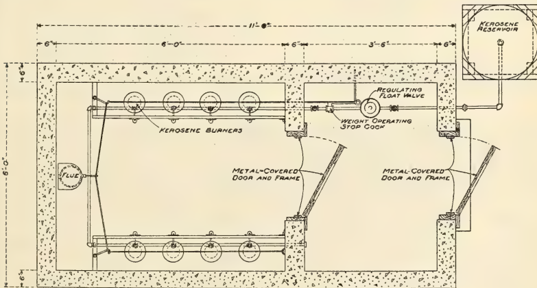
FIG. 9.—Plan of gas-generating room
