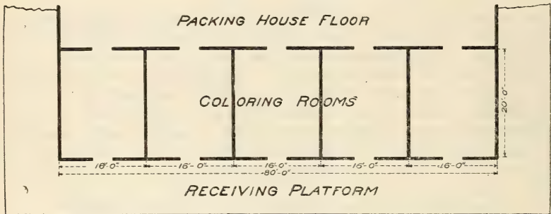
Fig. 7.—Diagram of floor plan, showing the arrangement of the coloring rooms in connection with the packing house
