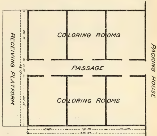
FIG. 8.—Diagram of floor plan, showing another arrangement of the coloring rooms in connection with the packing house
