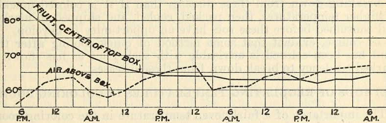
FIG. 2.—Diagram showing the air and fruit temperatures in the coloring room during experiment 3
