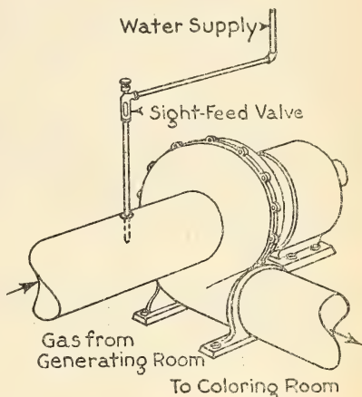
FIG. 3.—Apparatus used for dropping water into the intake of the exhaust fan
