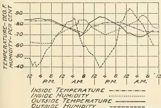
FIG. 4.—Diagram showing the temperature and humidity of the air inside the coloring room humidified by dropping water into the fan intake as compared with outside conditions
