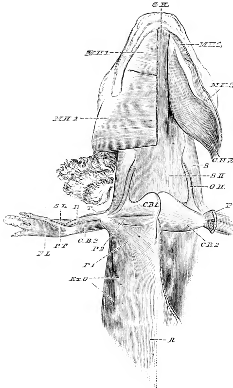
FIG. 67—Muscles of Ventral Surface of Menobranchus . On the right side, superficial muscles; on the left side, deeper muscles, the mylo-hyoidei, pectoralis, and external oblique being removed. Also superficial flexor muscles of right pectoral limb of Menobranchus . B , biceps; CB 1 and CB 2 , coraco-brachialis; CHE , cerato-hyoideus externus; EO , external oblique; FL , flexor longus; GH , genio-hyoideus; MH 1 and MH 2 , mylo-hyoideus; OH , omo-hyoideus; P , P 1 , and P 2 , pectoralis; R , rectus; S , subclavius; SH , sterno-hyoideus; SL , supinator longus; T , triceps.
