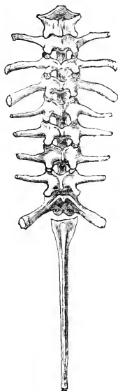
FIG. 30.—Backbone of the Frog (dorsal aspect).
