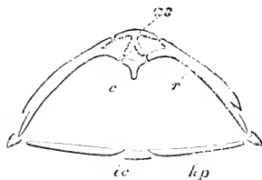
FIG. 23.—Diagram of a vertical section of both Carapace and Plastron of a Tortoise, made transversely to the long axis of the skeleton. c , vertebral centrum; ns , neural spine which expands above into a median dorsal scute; r , rib which forms one mass with a lateral scute and terminates at a marginal plate; ic , interclavicular scute; kp , hyo-sternal scute.
