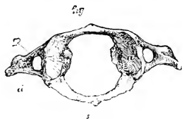
FIG. 34.—The Atlas Vertebra of Man. s , rudiment of neural spine; t , tubercular process; p , capitular process; a , articular surface for skull; hy , plate of bone holding the place of a cranium, and articulating with the odontoid process of the axis vertebra.
