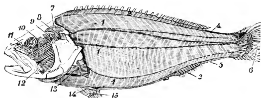
FIG. 59.—Superficial Muscles of the Perch. The fin-rays of all the fins are cut off. 1, great lateral muscle, showing the numerous vertical tendinous intersections slightly but variously inflected; 2, small superficial muscles inserted into the fin-rays of the dorsal and ventral fins; slender longitudinal muscle running (in the interval of the summits of the two great lateral muscles) between the dorsal and caudal fins; 5, similar muscle on the ventral margin, which also appears between the anal and ventral fins; 6, small radiating muscles of the caudal fin; 7, part of the great lateral muscle inserted into the skull; 8 and 9, elevators of the operculum; 10, elevator of the palato-quadrata arch; 11 and 12, muscular mass by which its contraction closes the jaws; 13, superficial muscles of the pectoral fin; 14 and 15, muscles of the ventral fin.
