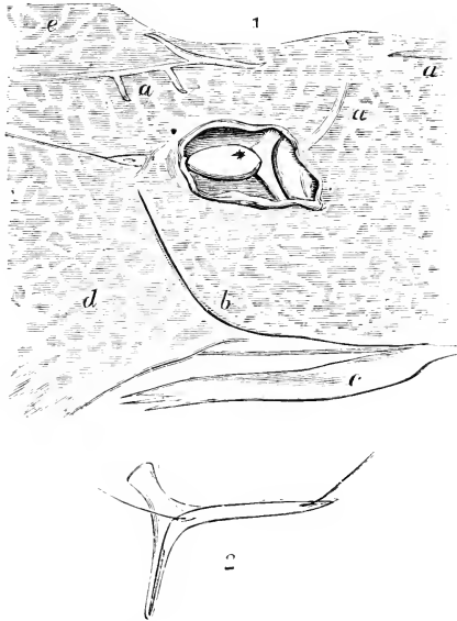
FIG. 7. — Poison Organ of Thalassophryne reticulata (after Günther). 1, Hind half of the head with the venous-sac of the opercular apparatus in situ . * Place where the small opening in the sac has been observed. a , Lateral line and its branches; b , gill-opening; c , central fin; d , base of pectoral fin; e , base of dorsal fin 2, Operculum, with the perforated spine.
