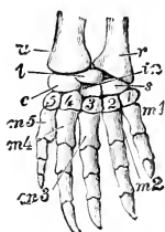
FIG. 50.—Dorsal surface of skeleton of right hand of the Tortoise, Chelydra (after Gegenbaur). c , cuneiforme; m , intermedium (or centrale); l , lunare; m 1 — m 5 , metacarpals; r , radius; s , scaphoides; u , ulna; 1—5, the five distal carpals, namely—1, trapezium; 2, trapezoides; 3, magnum; 4 and 5, divided unciforme.
