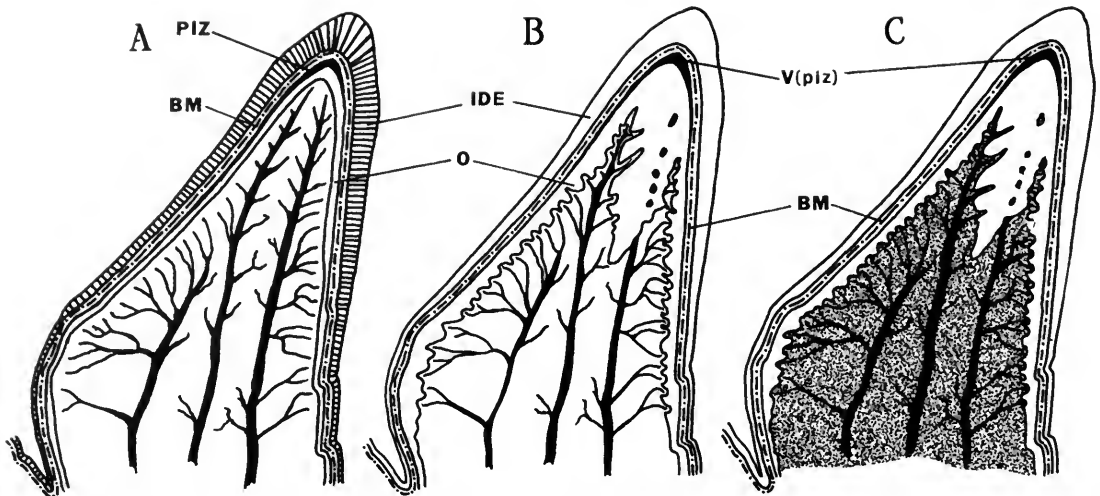
FIG. 10. Diagrammatic presentation of three (inferred) stages in the development of orthotrabecline in Petalodus (see text). BM, basement membrane; IDE, inner dental epithelium; O, orthodontine; PIZ, peripheral initial zone; V(piz), vitrodentine (mineralized peripheral initial zone).
