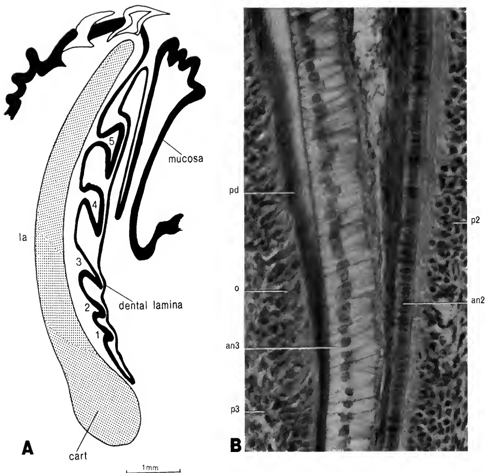
FIG. 2. A, Squalus acanthias . Section across lower jaw to show the dental lamina with its five tooth germs. The older replacement teeth are protected by a fold of the mucosa. cart, cartilage; la, labial. (After Peyer, 1968, pl. 8b; from Zangerl, 1981, fig. 19A. Reproduced by permission of Gustav Fischer Verlag.) B, Prionace glauca . Portion of a labiolingual, vertical section through a cross row of tooth anlagen in the lower jaw. Note the different sizes of the ameloblasts in tooth anlagen 2 and 3. o, odontoblasts; p2 and p3, mesenchymal cells within tooth germs 2 and 3; pd, predentine. Original magn. 333:1. (From Peyer, 1968, pl. 20b. © 1968 by The University of Chicago. All rights reserved.)
