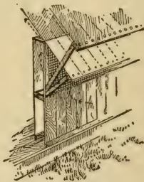
Showing Section of Draft Proof Ventilated Screened Wall.
