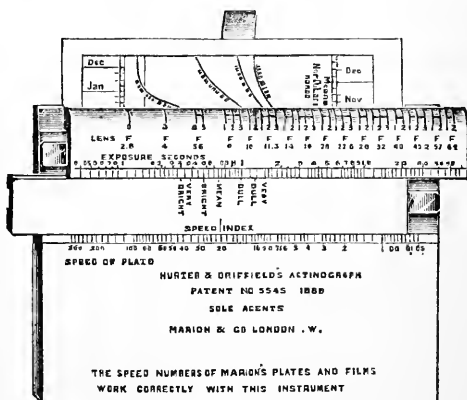
FIG. 13.—THE ACTINOGRAPH.
