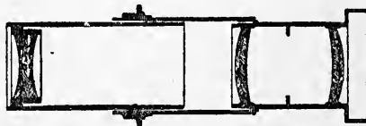
FIG. 10.—A TYPICAL TELEPHOTOGRAPHIC LENS.
