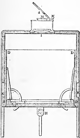
Horizontal section.
