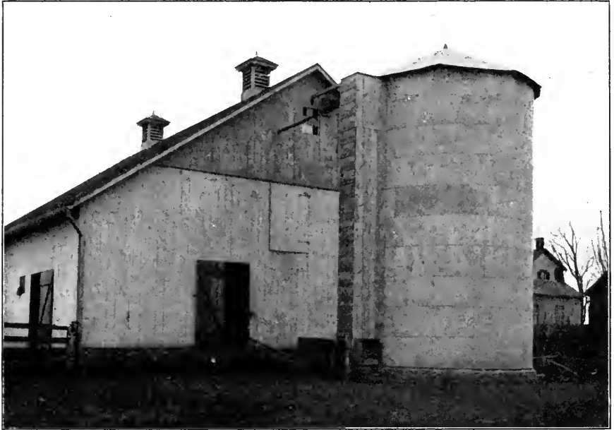
CUT 7.—WHERE NECESSARY TO FILL HAY LOFT FROM END OF BARN AT WHICH SILO IS LOCATED, A MOVABLE TRACK AND CAR MAY BE USED TO CARRY SILAGE TO MANGER.
