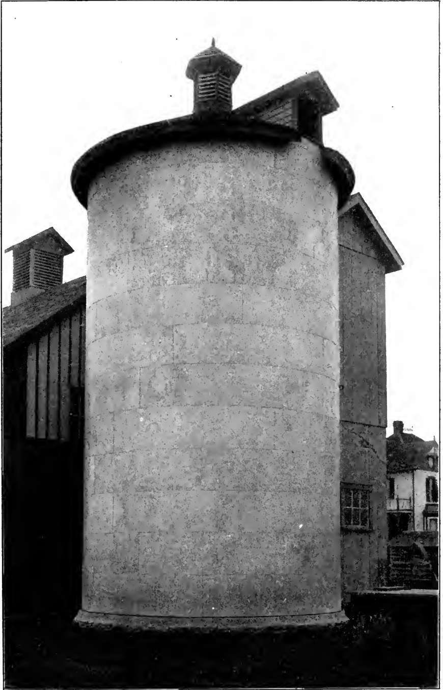
CUT 25.—SAME CONSTRUCTION AS SHOWN IN CUT 22; SHEETED WITH HALF-INCH LUMBER TO A HEIGHT OF SIX FEET AND COVERED WITH GALVANIZED IRON. AN EXPENSIVE COVERING BUT DURABLE AND SAVES PAINTING
