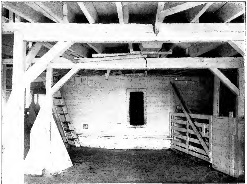
CUT 27.—SILO IN CENTER OF BARN SHOWN IN CUT 26. UPPER PORTION IN HAY LOFT, LOWER PORTION IN COW STABLE.
