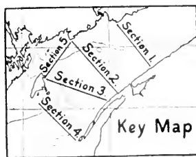
Plate IX. Salinity sections in the Bay of Fundy in August, 1919.
