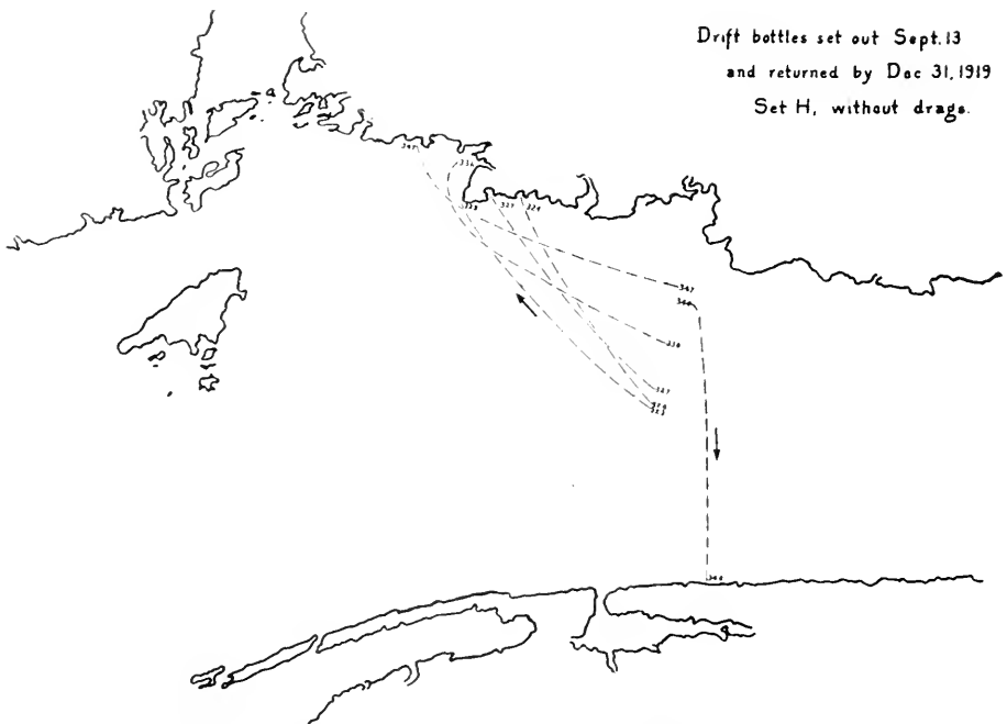
Fig. 9. Drift bottles of Set II. Chart showing where bottles set on the northwestern side of the Bay of Fundy were found.
