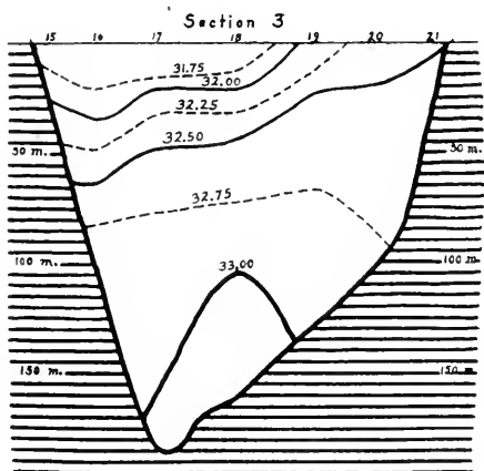
Plate IX. Salinity sections in the Bay of Fundy in August, 1919.
