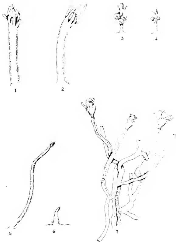
Figs. 1-6. Hydractinia laevispina .
