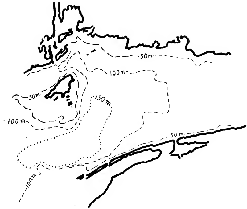
Figure 17. Depths in the lower half of the Bay of Fundy.
