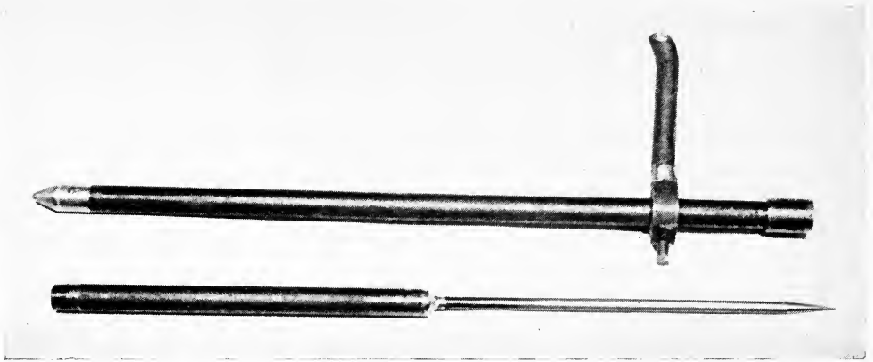
Fig. 15. Probe for locating pocket gopher tunnels to insert poisoned baits. The shaft may be in one piece or divided by a pipe coupling for convenience in carrying when not in use.
