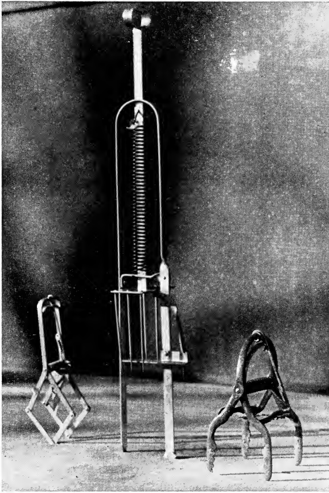
Fig. 19. Mole traps, as set for use. Left , choker-loop (Nash); center , spear (Reddick); right , lateral jawed (Out-o'-Sight).
