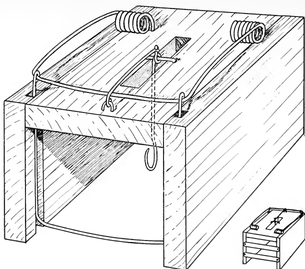
Fig. 7. Trap for ground squirrels (made from wooden pocket gopher trap) as set; smaller figure shows rear of trap.
