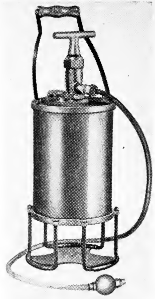
Fig. 5. The Demon Rodent Gun for pumping liquid carbon disulfide into rodent burrows.
