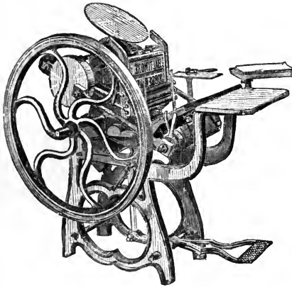
The "Baltimore" Jobber.
