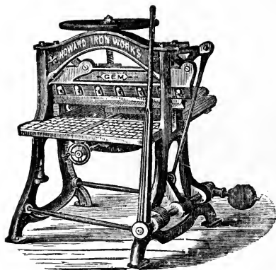
Gem Paper Cutter.
