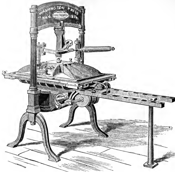
"Washington" Hand Press.
