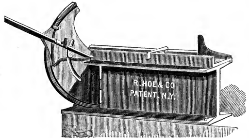
Horizontal Mitering Machine.
