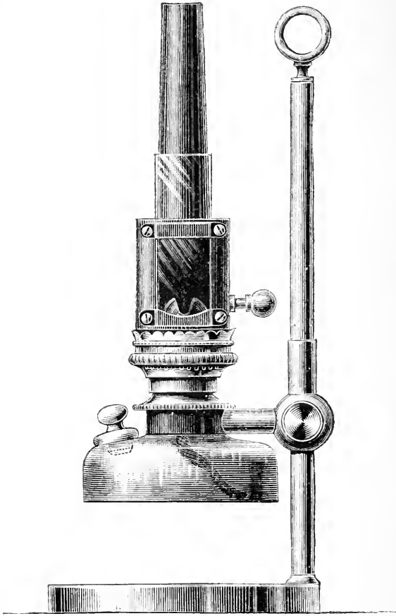
FIG. 3.—Baker's microscope-lamp.
