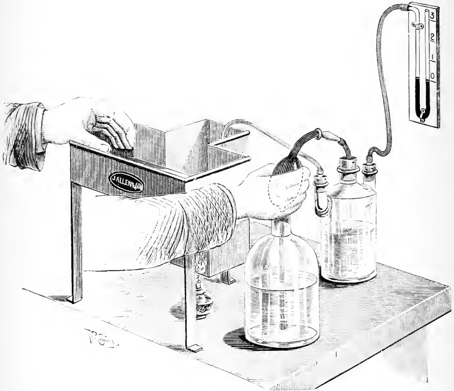
FIG. 34.—Injecting bath, author's pattern.
