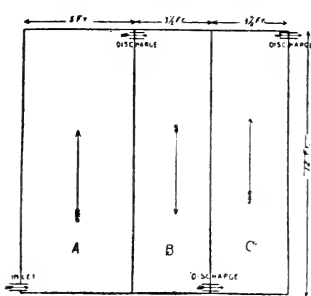
Fig. 45.—Cross Section of Septic Tank.
