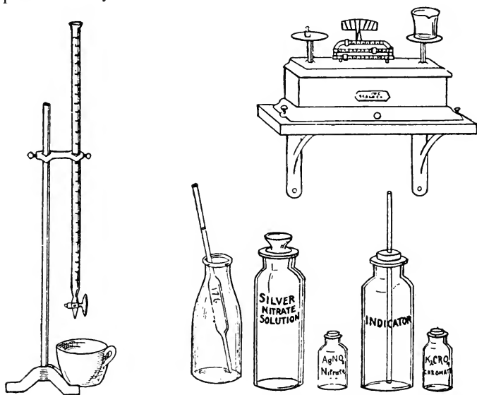
Apparatus needed in salt determination.
