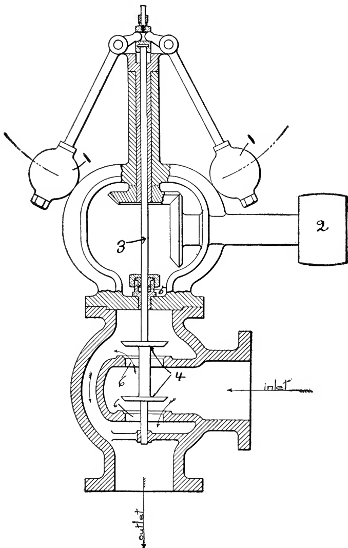
Fig. 83.—Governor.
