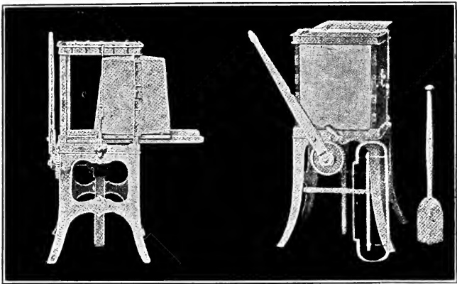
Fig. 29.—Butter printers for printing butter from square boxes and from tubs after thorough chilling in the refrigerator.
