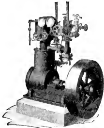
Belt Driven Single- Acting Com- pressor
