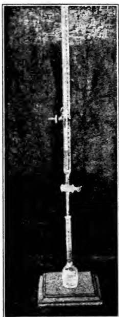
Fig. 11. Burette method.
