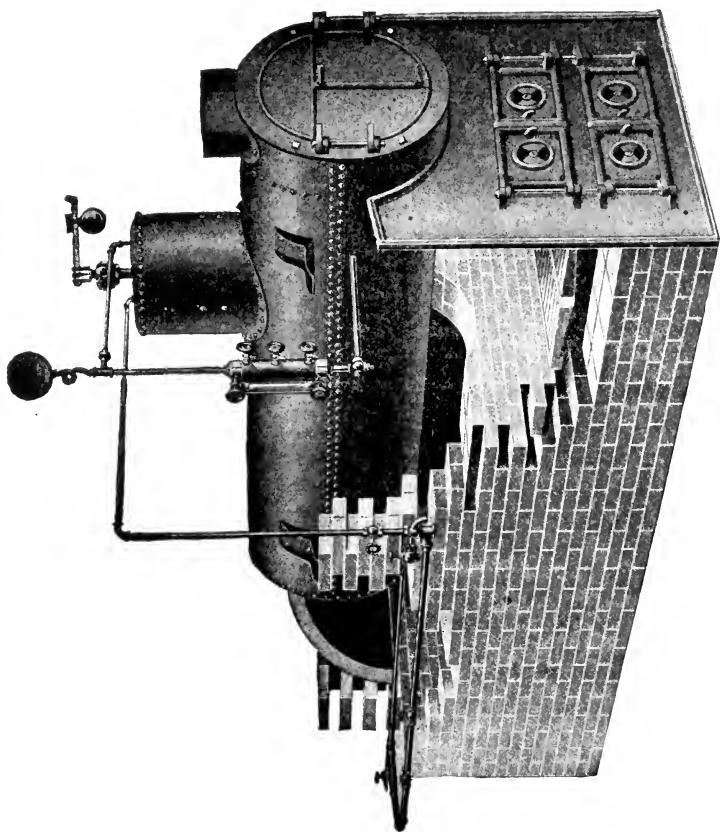
Fig. 75. — Firetube boiler.
