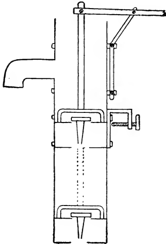
Fig. 27.—Cream pump.
