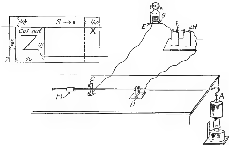
FIG. 163. An electric alarm for an incubator.
