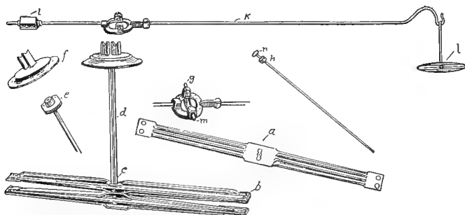
FIG. 157.—Various parts of a thermostat. (See body of text for description.)
