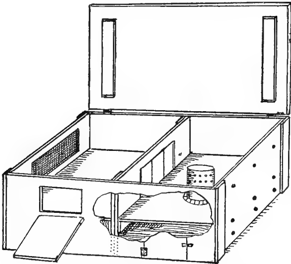
FIG. 169.—A home-made brooder. (See description in text.)
