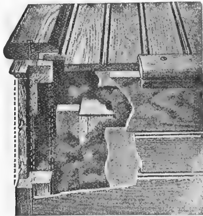
FIG. 154.—A view showing insulation of a small incubator.
