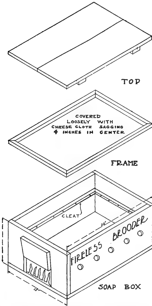
FIG. 172.—A fireless brooder made out of an ordinary soap box. The heat cushion is a bag of chicken feathers or a woolen blanket. Holes in the sides of the box give ventilation. (Pennsylvania Department of Agriculture.)
