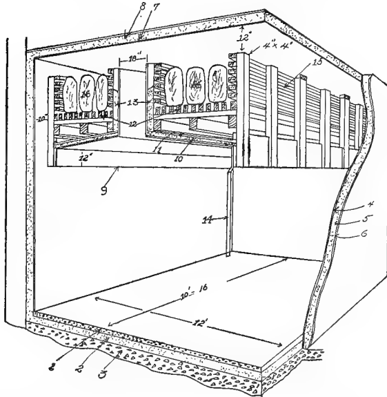
FIG. 199.—A typical ice chilled room—with overhead bunker. 1, Concrete; 2, cork; 3, concrete base; 4, \frac{1}{4} -inch rough and \frac{1}{4} -inch finish coat; 5, 4-inch cork; 6, \frac{1}{4} -inch rough \frac{1}{4} -inch finish; 7, \frac{1}{2} -inch plaster; 8, 5-inch cork; 9, 2-inch cork; 10, 2-inch cork; 11, drip pan; 12, removable racks; 13, 2-inch cork; 14, drain pipe; 15, ice rack; 16, ice.
