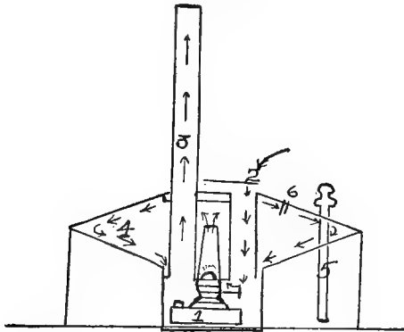
FIG. 170.—A small oil-burning hover sold on the market. 1, The lamp; 2, the intake flue; 3, the draft pipe; 4, the radiating drum; 5, the thermometer; 6, peep hole.
