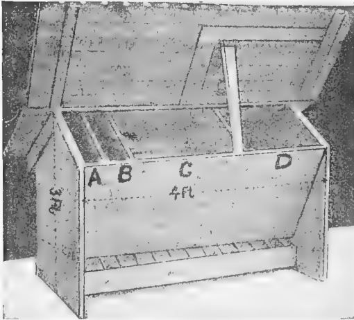
FIG. 107.—An outdoor mash hopper. The four compartments A , B , C , and D are for use as in Fig. 106, d . The dimensions are given on the box. It is covered with rubberoid.
