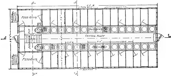
Double Brooder House
