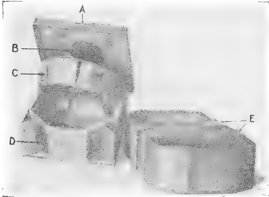
FIG. 175.—The H and D brooder sold on the market: A , Celliform construction of ventilation, exit of foul air; B , opening through which foul air passes; C , hover showing non-ravelling felt; D , door from hover chamber to non-crowding yard; E , sliding boards to adjust yard.
