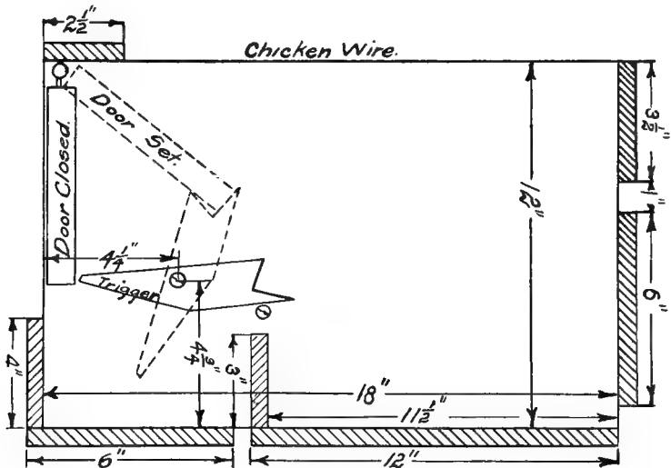
FIG. 210.—Side sectional view of a trap-nest.
