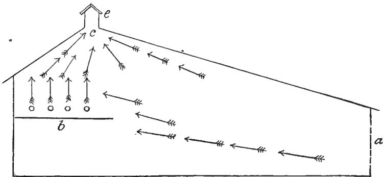
FIG. 59.—If a house be constructed as indicated the vitiated air would rise at the highest point in the house, which is at c , and unless provided with a ventilator would stagnate there. With the ventilator the air enters the house at a (an open front), passes backward over the roosts at b , and takes an upward course and out the ventilator at e .
