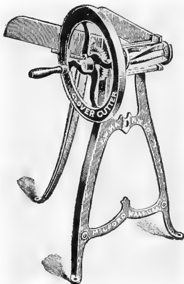
FIG. 100.—A green feed cutter sold on the market.
