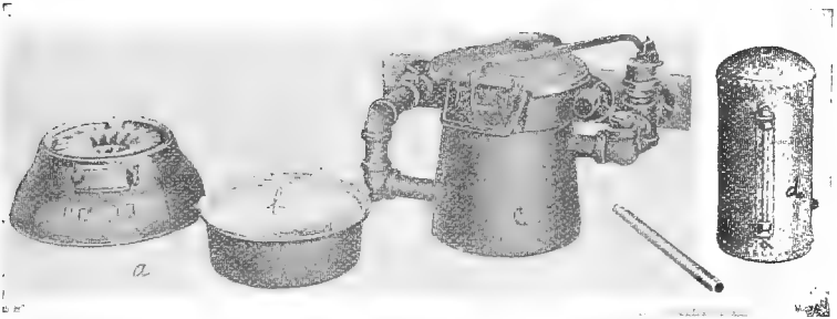
FIG. 162.—The parts of a heater in a giant incubator: a , The base and grate; b , the brick ring; c , heater, water-pot, and top; d , pipe tank and gauge-glass.
