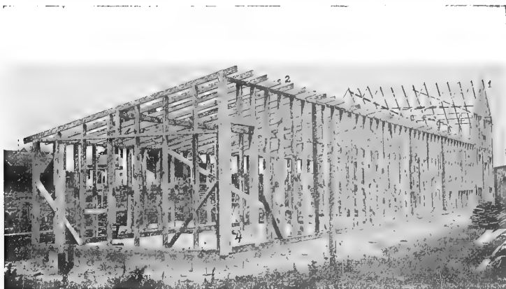
FIG. 85.—The frame work of the superstructure, showing the main building and one wing: 1, The main building; 2, the wing; 3, the foundation; 4, the cement floor seen through the end door of first compartment; 5, one of the 4 by 4 inch sills fastened by a bolt embedded in the concrete.
