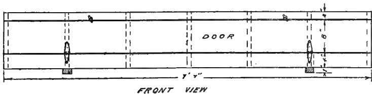
FIG. 215.—The construction of hen's nests.
