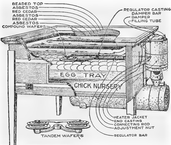
FIG. 153.—A diagram showing the parts of a small incubator. (St. Helms. Inc. Co.)
