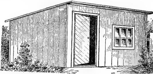
FIG. 113.—A cheap and convenient duck house. The floor is dirt and level, and covered 6 inches deep with clean straw on which the ducks roost.
