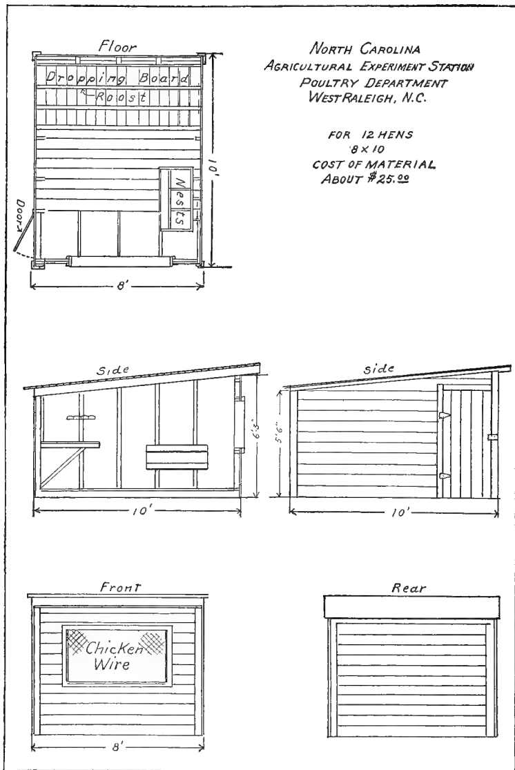
FIG. 73.—Photograph of a blue print from the North Carolina Exp. Station. This is a house suitable for the town lot or for the boys and girls poultry clubs.
