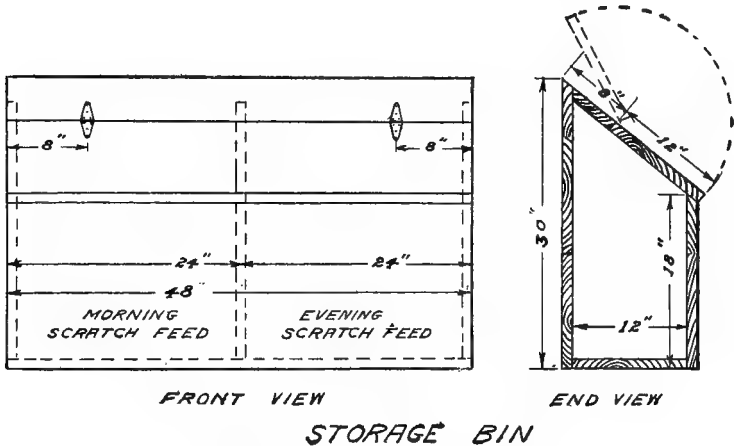
FIG. 213.—A grain storage bin.
