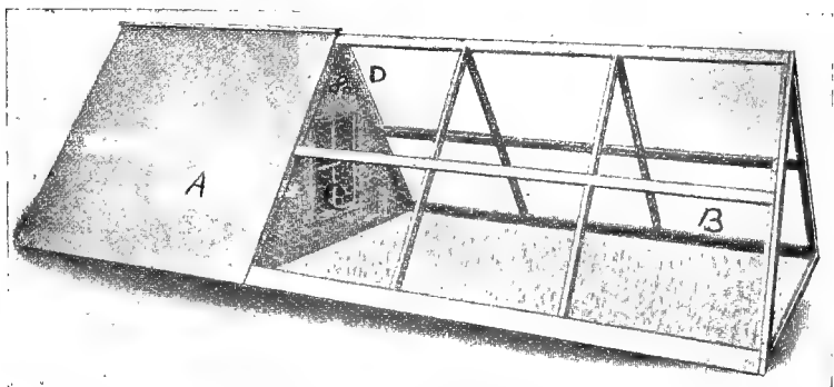
FIG. 150.—A cheap and convenient boys and girls poultry club house and run for sitting and brooding: A , The house; B , the wire-netting run; C , the door to the coop; D , the ventilating holes.
