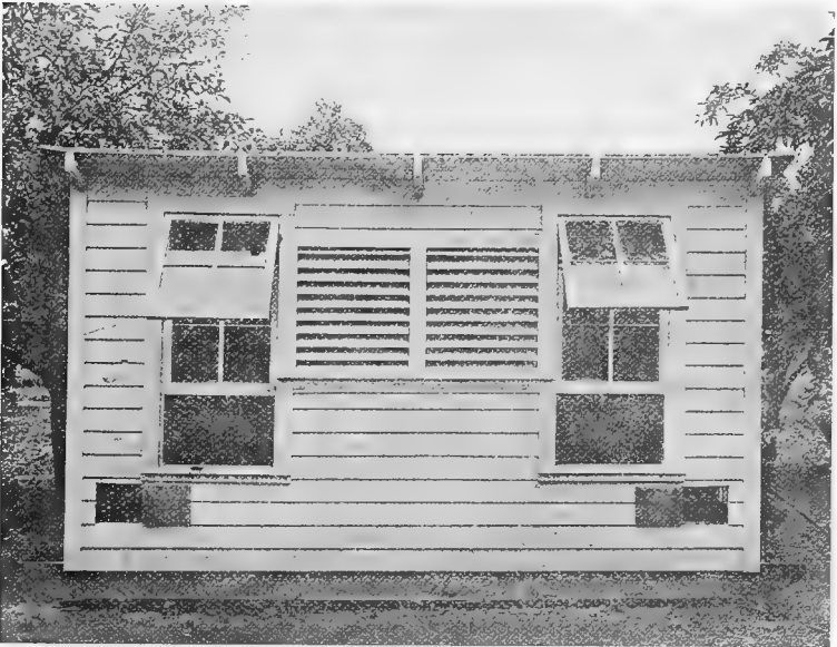
FIG. 96.—A portable poultry house. Note at a the sled runners, New York State Exper. Sta.
