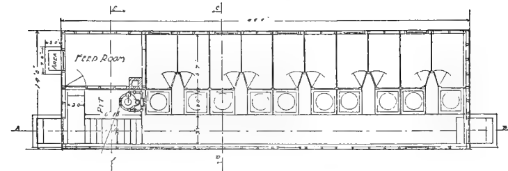
Single House with Alley Between Brooders
