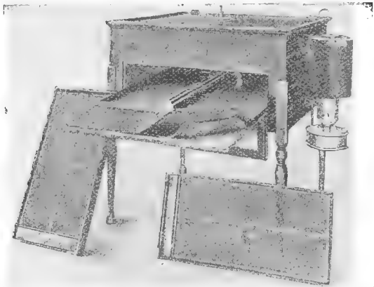
FIG. 156. An incubator ready for use. Showing egg-tray, nursery tray, lamp, and thermoregulator.
