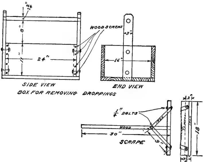
Fig. 214.—Dropping box and dropping board scrape.
