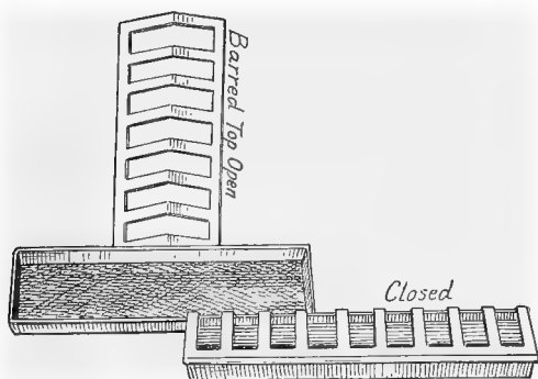
FIG. 93.—Good commercial feed- and water-troughs. The slatted top keeps the birds from getting their soiled feet in the feed.
