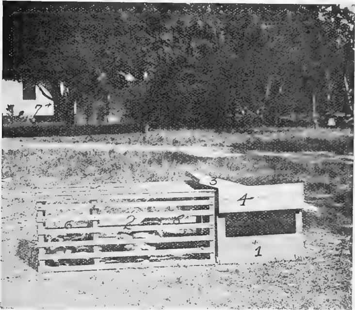
FIG. 148.—A combination sitting and brooding coop. 1, Side view of the coop; 2, the extension run; 3, the roof; 4, the door to the coop; 5, the compartment for the hen; 6, the compartment in which to feed the chicks; 7, shade tree necessary in chick raising. See page 412 for construction.
