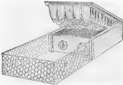
FIG. 176.—A commercial fireless brooder sold on the market: a , Strips of felt; b , the opening through which the chicks enter to the yard c .
