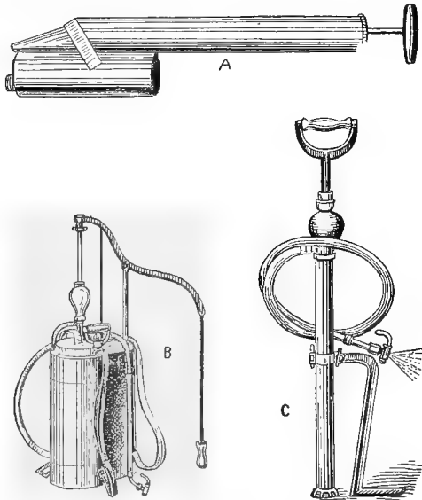
FIG. 95.—Three useful spray pumps: A , A small hand pump; B , a knapsack type; C , the best type force spray pump. With this pump the spray can be driven into the cracks and crevices which is necessary in successful disinfection.
