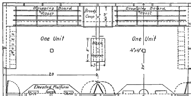
Floor Plan
