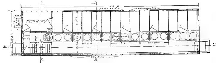
Single Brooder House
