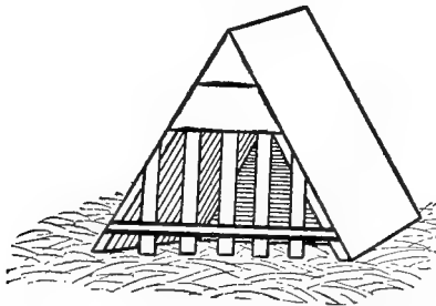
FIG. 152.—A cheap and convenient A-house for a hen and her brood.
