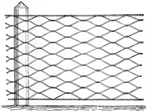
FIG. 69.—Six-sided mesh poultry wire. This is a poor netting, and to hold it in shape in the fence it is necessary to make a frame for it so that it is possible to staple it on all four sides of the panels.
