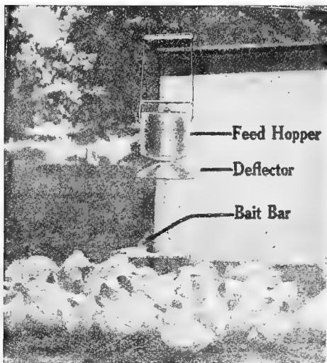
FIG. 116.—An exerciser sold on the market. The birds picking at the bait in the small cylinder close to the ground cause some grains of feed to drop out onto the deflector and to the ground.
