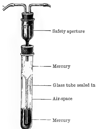
FIG. 12.—SCHENK'S THERMO-REGULATOR.
