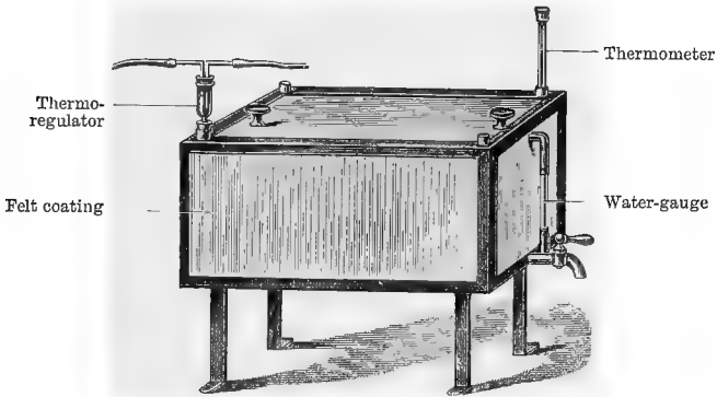
FIG. 11.—INCUBATOR.
