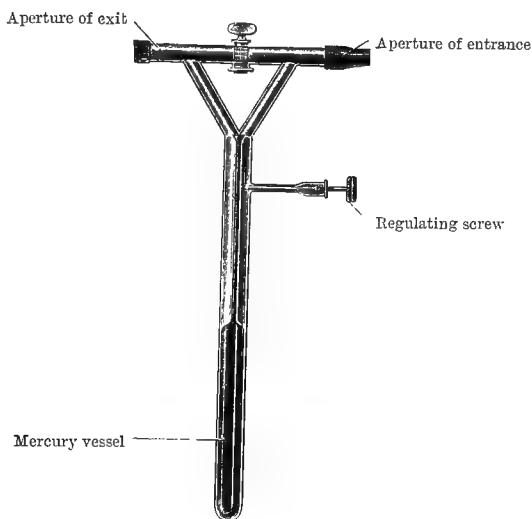
FIG. 13.—ALTMANN'S THERMO-REGULATOR.
