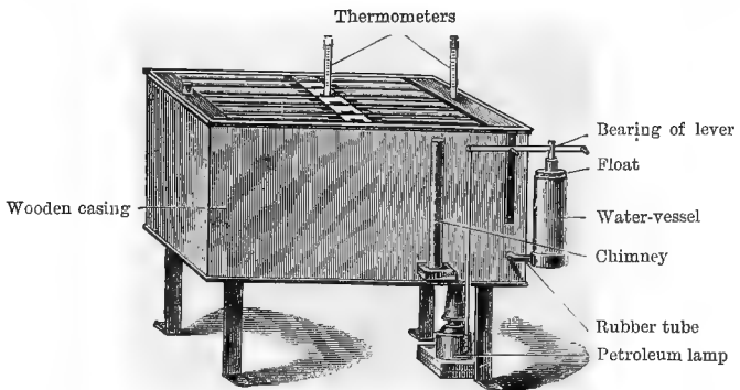
FIG. 14.—BAUMEIER'S PETROLEUM INCUBATOR.
