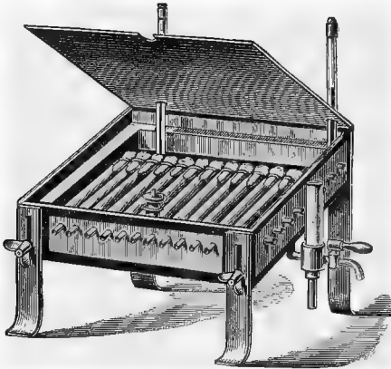
FIG. 23.—APPARATUS FOR THE INSPISSATION OF BLOOD SERUM.
