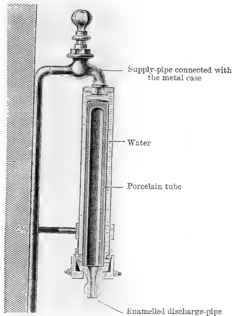
FIG. 44.—KAOLIN FILTER, ON THE CHAMBERLAND-PASTEUR SYSTEM.
