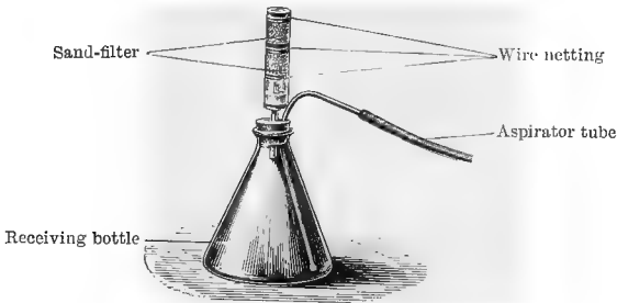
FIG. 33.—PETRI'S SAND-FILTERING APPARATUS.
