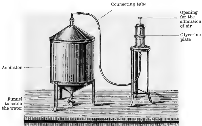
FIG. 28.—POUCHET'S AËROSCOPE.
