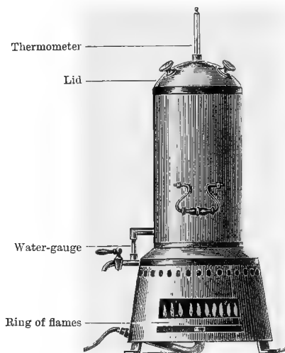
FIG. 10. —KOCH'S STEAM STERILISER.
