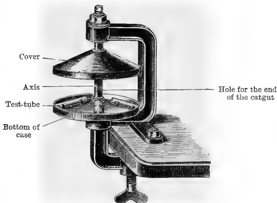
FIG. 21.—GÄRTNER'S CENTRIFUGE.
