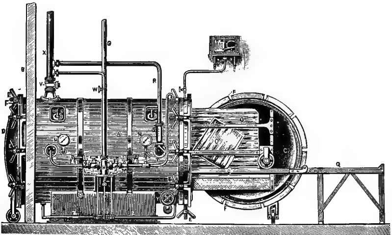
FIG. 34.—EQUIFEX DISINFECTOR.
