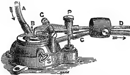
FIG. 7.—EXCELSIOR GAS-VALVE.
