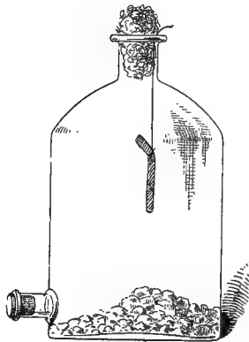
FIG. 20.—DRYING BOTTLE.
