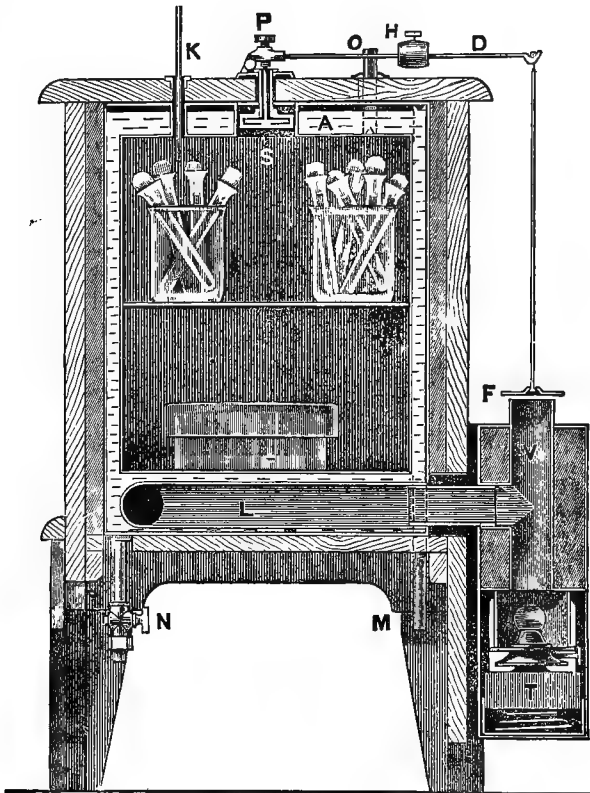
FIG. 8.—INCUBATOR HEATED BY A LAMP.
