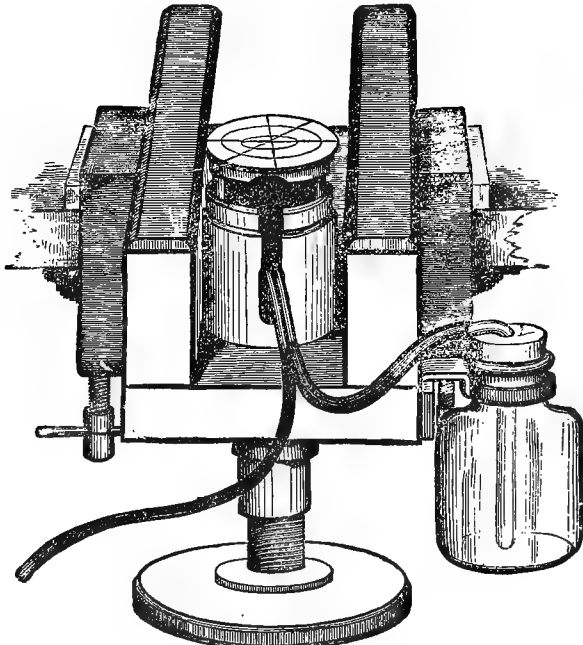
FIG. 5.—FREEZING MICROTOME.
