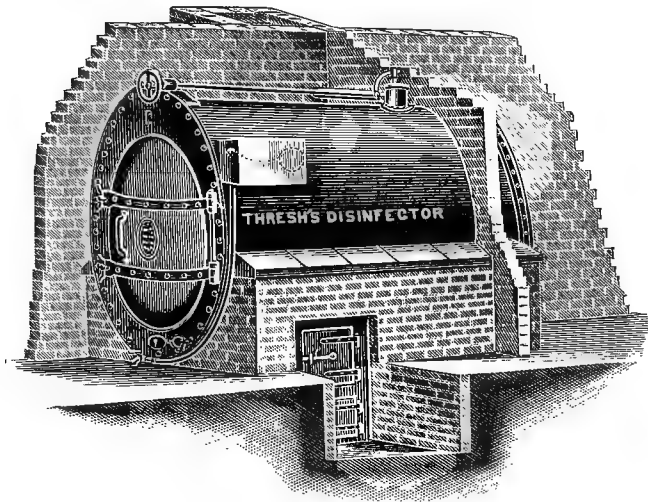
FIG. 35.—THRESH'S DISINFECTOR.
