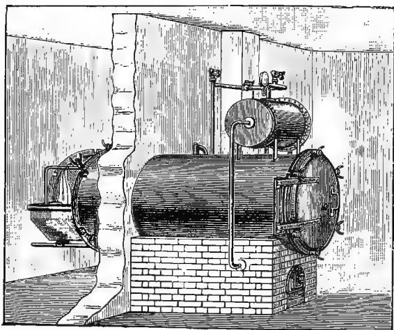
FIG. 36.—RECK'S DISINFECTOR.
