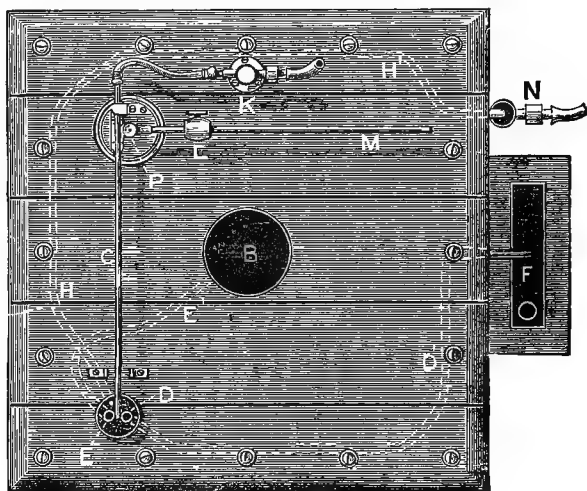
FIG. 9.—PLAN OF COOL INCUBATOR.
