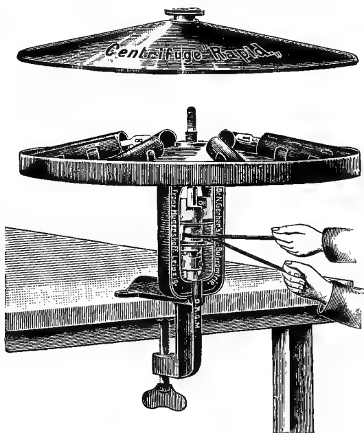
FIG. 10.—CENTRIFUGAL MACHINE.
