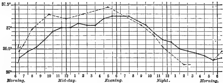
FIG. 340.—Variations of the daily temperature in health during 24 hours: L., after Liebermeister; J., after Jürgenson (from Landois).
