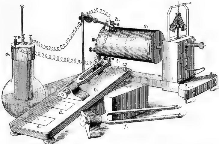
FIG. 166. —Marey's chronograph as applied to revolving cylinder (after McKendrick). a , galvanic element; b , wooden stand bearing tuning-fork (two hundred vibrations per second); c , electro-magnet between limbs of tuning-fork; d, e , positions for tuning-forks of one hundred and fifty vibrations per second; f , tuning-fork lying loose, which may be applied to d ; g , revolving cylinder; h , electric chronograph kept in vibration synchronous with the tuning-fork interrupter. The current working the electro-magnet from a is interrupted at i . Foucault's regulator is seen over the clock-work of the cylinder, a little to the right of g .
