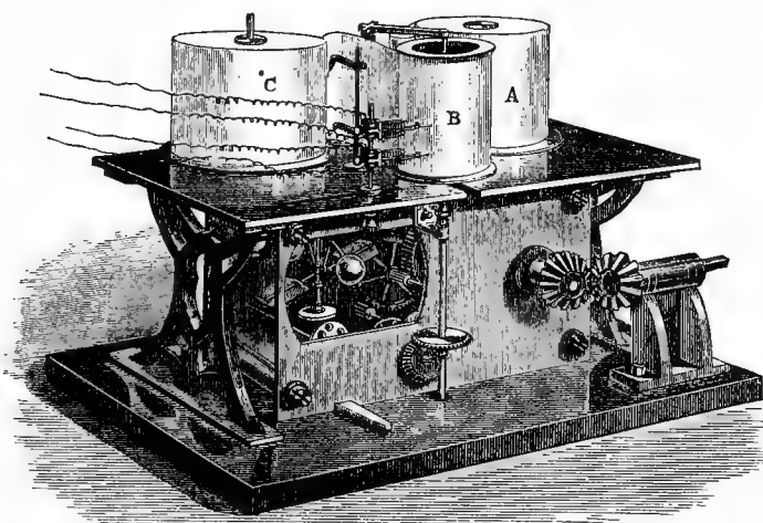
FIG. 208.—Large kymograph, with continuous roll of paper (Foster). The clock-work machinery unrolls the paper from the roll C, carries it smoothly over the cylinder B, and then winds it up into the roll A. Two electro-magnetic markers are seen in position recording intervals of time on the moving roll of paper. A manometer may be fixed in any convenient position.
