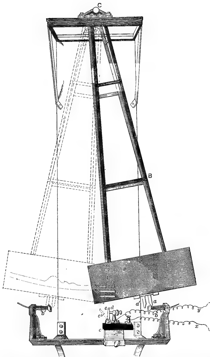
FIG. 177.—Diagrammatic representation of the pendulum myograph. The smoked-glass plate, A , swings with a pendulum, B . Before an experiment is commenced the pendulum is raised up to the right and kept in position by the tooth, a , catching on the spring-catch, b . On depressing the catch, b , the glass plate being set free swings into the new position indicated by the dotted lines, and is held there by the tooth, a' , meeting the catch, b' . In the course of its swing the tooth, a , coming into contact with the projecting steel rod, c , knocks it to one side, into the position indicated by the dotted line, c' . The rod, c , is in electric continuity with the wire, x , of the primary coil of an induction machine. In like manner
