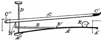
FIG. 218.—Diagrammatic schema showing the essential part of the instrument when in working order. The knife-edge, B' , of the short lever is in contact with the writing-lever, C . Every movement of the steel spring at A' , communicated by the arteries, will be imparted to the writing-lever (Byrom Bramwell).
