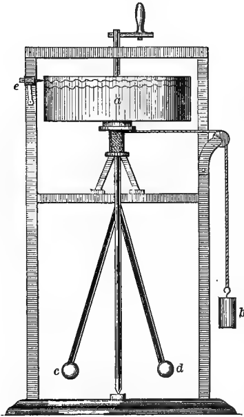
FIG. 164.—Original chronometer, devised by Thomas Young, for measuring minute portions of time (after McKendrick). a , cylinder revolving on vertical axis; b , weight acting as motive power; c , d , small balls for regulating the velocity of the cylinder; e , marker recording a line on cylinder.
