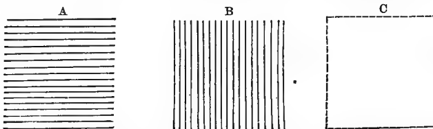
FIG. 431.—Illustrates illusions as to size. In A the height seems at first greater than the breadth, though they are equal: the reverse in B; while C appears to cover a less area than either of the others (after Bernstein).
