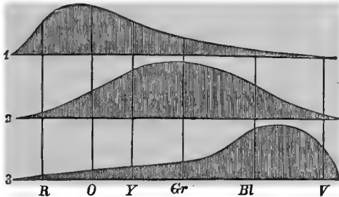
FIG. 427.—Illustrates the Young-Helmholtz theory of color-vision. The letters in the lower line indicate colors of spectrum in natural order. 1. denotes the "red"; 2, "green"; 3, "violet" primary-color sensation. The diagram shows by the height of the curve in each instance to what extent the primary-color sensations are respectively excited by vibrations of different wave-lengths (after Bernstein).
