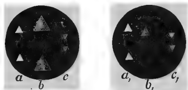
FIG. 411.—Purkinje's images. a b c during negative, a, b, c , during positive accommodation (after Landolt).
