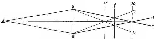
FIG. 415.—Diagram to illustrate chromatic aberration (after Foster).
