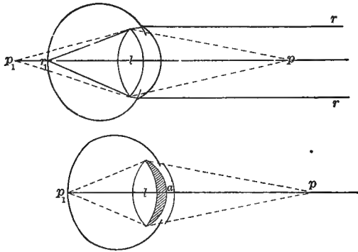
FIG. 416.—Diagrams to illustrate conditions of refraction in normal eye when unaccommodated (passive, or negatively accommodated), and when accommodated for "near" objects (after Landois).
