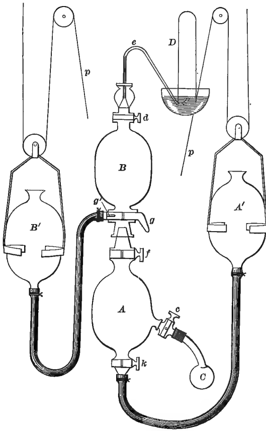
FIG. 315.—Diagrammatic illustration of Ludwig's mercurial gas-pump. A and B are two glass globes, connected by strong India-rubber tubes, with two similar glass globes, A' and B' . A is further connected by means of the stop-cock c with the receiver C , containing the blood (or other fluid) to be analyzed; and B , by means of the stop-cock d and tube e with the receiver D , for receiving the gases. A and B are also connected with each other by means of the stop-cocks f and g , the latter being so arranged that B also communicates with B' by the passage g' . A' and B' being full of mercury, and the cocks k , f , g and d being open, but c and g' closed, on raising A' by means of the pulley p the mercury of A' fills A , driving out the air contained in it into B , and so out through e . When the mercury has risen above g , f is closed; and g' being opened, B' is in turn raised till B is completely filled with mercury, all the air previously in it being driven out through e . Upon closing d and lowering B' , the whole of the mercury in B falls into B' , and a vacuum consequently is established in B . On closing g' but opening g , f , and k , and lowering A' , a vacuum is similarly established in A and in the junction between A and B . If the cock c be now opened, the gases of the blood in C escape into the vacuum of A and B . By raising A' after the closure of c and opening of d , the gases so set free are driven from A into B , and by the raising of B' from B through e into the receiver D , standing over mercury. (After Foster.)
