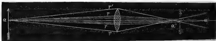
FIG. 414.—Illustrating spherical aberration (after Le Conte). The best image is formed at S, S' , but is not perfectly sharply defined even here.
