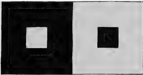
FIG. 428.—Illustrates irradiation. The white patch in the dark ground seems larger than the dark one in the light ground (after Bernstein).
