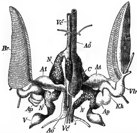
FIG. 227.—Circulatory and excretory organs of the cuttle-fish ( Sepia officinalis ), viewed from the dorsal side (after Hunter). Br , gills; C , ventricle; Ao and Ao' , anterior and posterior aorta; V , lateral vein; Vc' , anterior vena cava; Vc'' , posterior vena cava; N , renal appendages of the veins; Vlr , advent branchial vessels (branchial arteries); Kh , branchial heart; Ap , appendage of the same; At , At' , auricles receiving the revehent branchial vessels (branchial veins).
