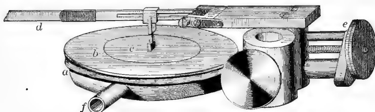
FIG. 175.—Tambour of Marey (after McKendrick). a , metallic case; b , thin India-rubber membrane; c , thin disk of aluminium supporting lever d , a small portion of which only is represented; e , screw for placing support of lever vertically over c ; f , metallic tube communicating with cavity of tambour for attachment to an India-rubber tube.
