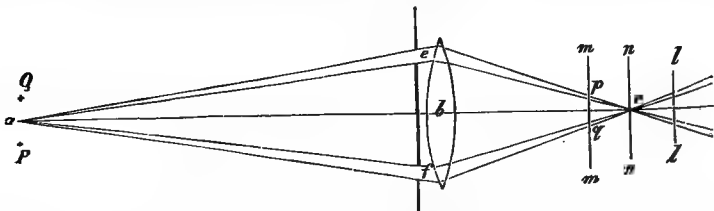
FIG. 410.—To explain Scheiner's experiment (after Bernstein). The object is at a ; the lens is represented by b ; and the retina may be at m, n, n, or l, l . The card with its holes, e, f , is directly in front of the lens. It is plain that, if the rays strike the retina in any way except as represented at c , double images must be formed. One or other of these will disappear according as the right or left hole of the card is stopped; which of them will depend on circumstances—i. e., as to whether the case is that figured at m, m or l, l .
