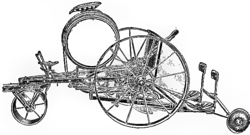
FIG. 145. — A transplating machine. Two operators or planters ride behind.
