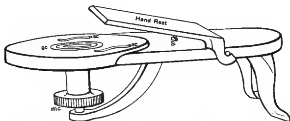
FIG. 191. TURN-TABLE FOR MAKING CELLS AND FOR SEALING COVER-GLASSES.
