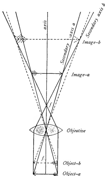
FIG. 83. TO SHOW THE RELATIVE POSITION OF THE OBJECT AND THE REAL IMAGE.
