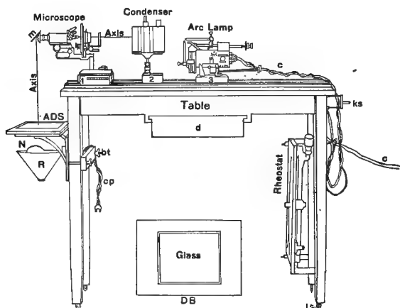
FIG. 247. DRAWING AND PROJECTION OUTFIT.
