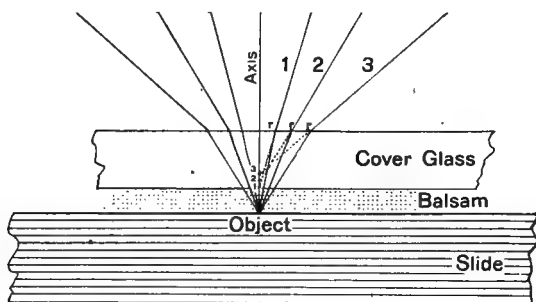
FIG. 169. SPHERICAL ABERRATION INTRODUCED BY THE COVER-GLASS.
