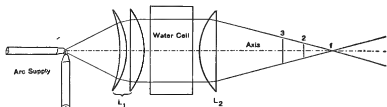
FIG. 121. ILLUMINATING OBJECTS OF VARIOUS SIZES IN MICRO-PROJECTION WITH THE MAIN CONDENSER ONLY.
