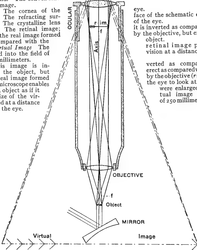
FIG. 20. COMPOUND MICROSCOPE WITH PROJECTED VIRTUAL IMAGE.
