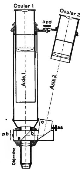
FIG. 53. IVES BINOCULAR ARRANGEMENT FOR ALL POWERS.
