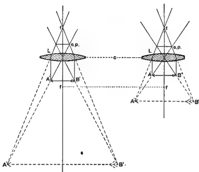
FIG. 15-16. VIRTUAL IMAGE WITH THE OBJECT NEAR TO AND FAR FROM THE PRINCIPAL FOCUS.
