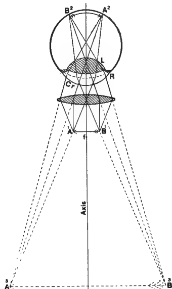
FIG. 182. PROJECTED VIRTUAL IMAGE OF A MAGNIFIER. (Simple Microscope or Ocular).
