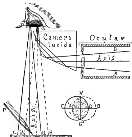
FIG. 81. WOLLASTON'S CAMERA LUCIDA.
