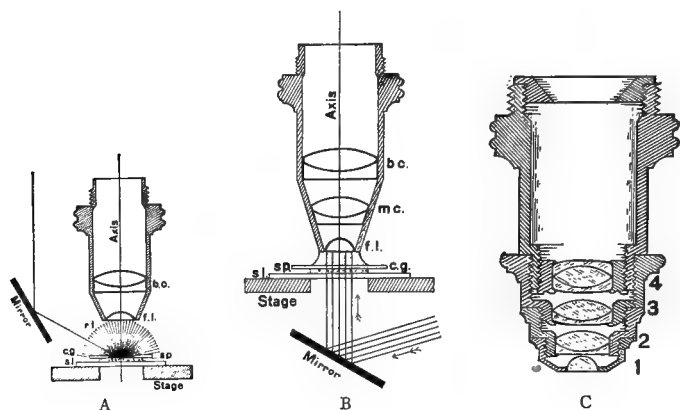
FIG. 21 A. LOW OBJECTIVE IN SECTION.
