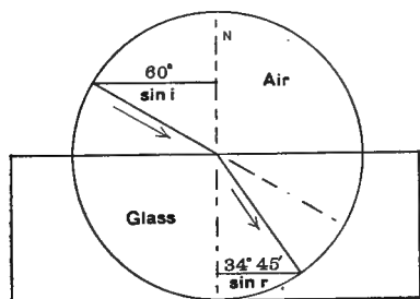
FIG. 155. REFRACTION OF LIGHT IN PASSING FROM AIR TO GLASS.
