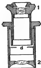
FIG. 137. PROJECTION OCULAR IN SECTION.
