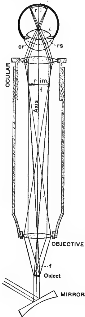
FIG. 3. A COMPOUND MICROSCOPE HELPING THE EYE TO FORM A RETINAL IMAGE OF A NEAR OBJECT.
