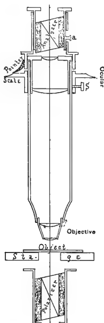
FIG. 150. MICRO-POLARISCOPE IN POSITION ON THE MICROSCOPE.
