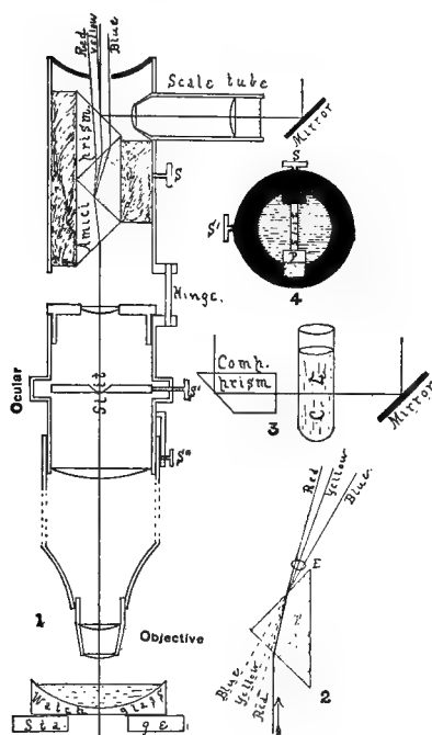
FIG. 145. DIAGRAM OF A DIRECT-VISION MICRO-SPECTROSCOPE.
