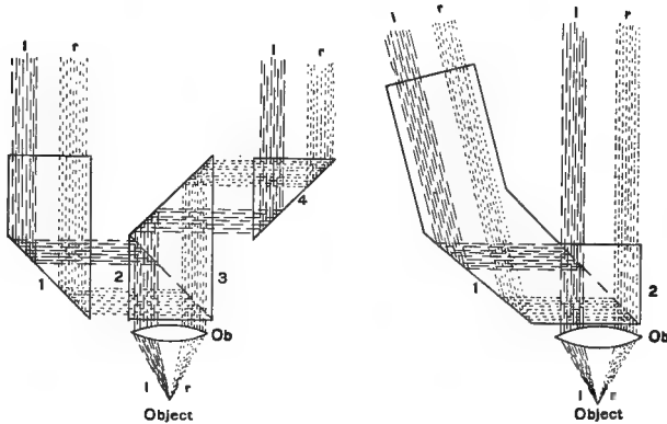
FIG. 54-55. PRISM ARRANGEMENT FOR TWO FORMS OF BINOCULARS FOR ALL POWERS.
