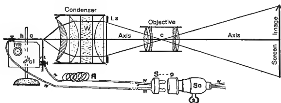
FIG. 110. MAGIC LANTERN WITH PROJECTED IMAGE.
