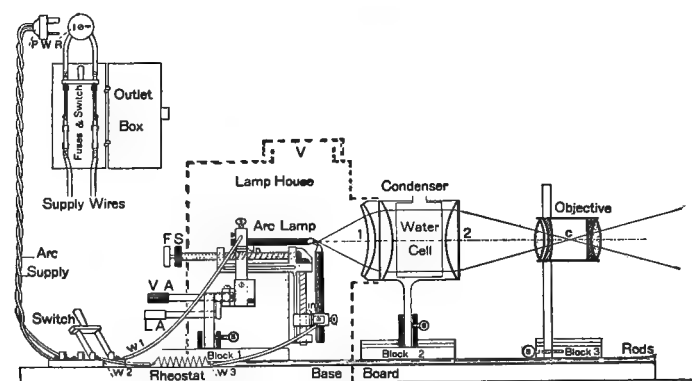
FIG. 122. PROJECTION APPARATUS SHOWING THE PARTS AND THE WIRING FOR AN ARC LAMP.
