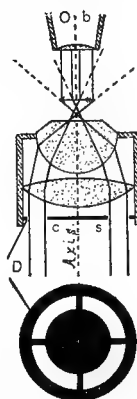
FIG. 47. DARK-GROUND ILLUMINATION BY A HOLLOW CONE OF LIGHT.
