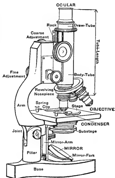
FIG. 25. LABORATORY COMPOUND MICROSCOPE WITH THE PARTS NAMED.
