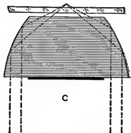
FIG. 50. CONDENSER FOR DARK-GROUND ILLUMINATION.
