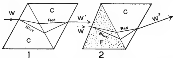
FIG. 172. ACHROMATISM BY COMBINING DIFFERENT KINDS OF GLASS.
