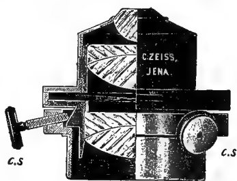
FIG. 40. ACHROMATIC SUBSTAGE CONDENSER WITH THE DIAPHRAGM BETWEEN THE COMBINATIONS.
