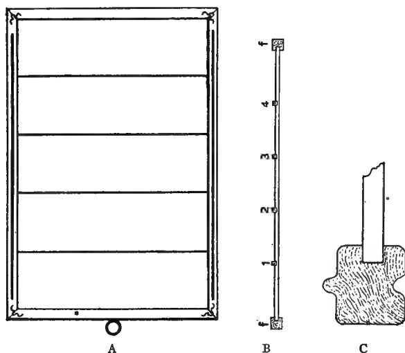
FIG. 207. SLIDE TRAY WITH COMPARTMENTS, AND WITH TONGUE AND GROOVE IN THE SIDE PIECES OF THE FRAME.
