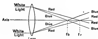
FIG. 171. CHROMATIC ABERRATION WITH COMPOSITE LIGHT.
