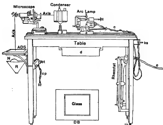
FIG. 109. PROJECTION MICROSCOPE, TABLE, AND ADJUSTABLE DRAWING SHELF. (Modified from Optic Projection).
