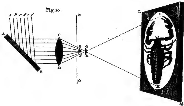
FIG. 119. DIAGRAM OF ADAMS' SOLAR MICROSCOPE. THIS ILLUSTRATES WELL THE ADVANTAGE OF SOME FORM OF PROJECTION MICROSCOPE FOR DEMONSTRATION PURPOSES.
