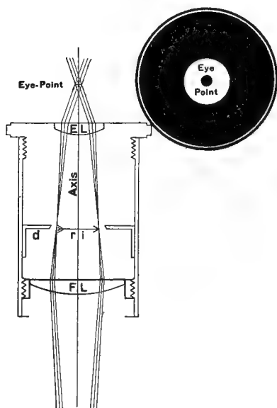
FIG. 24. HIGH-POWER HUYGENIAN OCULAR.
