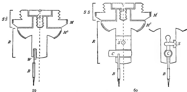
FIG. 59-60. MARKERS FOR MICROSCOPICAL SPECIMENS.
