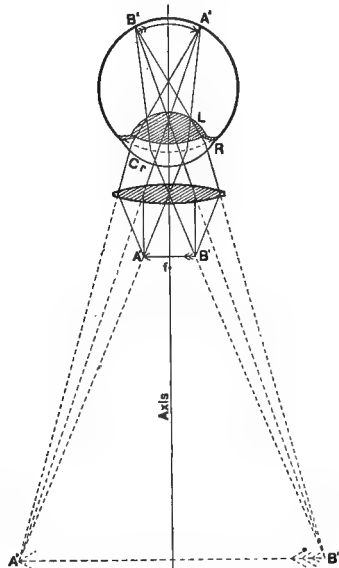
FIG. 77. SIMPLE MICROSCOPE WITH THE VIRTUAL IMAGE AT 250 MM. FROM THE EYE.
