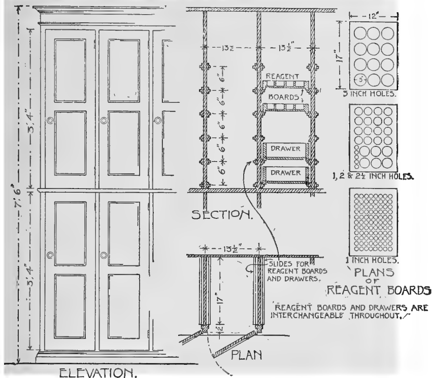
FIG. 208. LABORATORY LOCKERS REAGENT BOARDS AND DRAWERS DESIGNED IN 1895.
