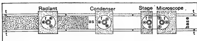
FIG. 132. HOME-MADE OPTICAL BENCH. (About \frac{1}{10} natural size. From Optic Projection).
