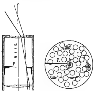
FIG. 62-63. POINTER OCULAR AND MICROSCOPIC FIELD.
