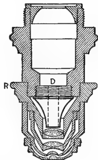
FIG. 48. HIGH-POWER OBJECTIVE WITH APERTURE REDUCING DIAPHRAGM FOR DARK-GROUND ILLUMINATION.
