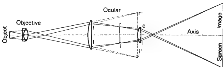
FIG. 183. DIAGRAM SHOWING THE RAYS AND IMAGES WHEN BOTH AN OBJECTIVE AND AN OCULAR ARE USED.
