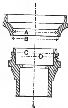
FIG. 64. ROYAL MICROSCOPICAL SOCIETY'S STANDARD SCREW FOR OBJECTIVES.
