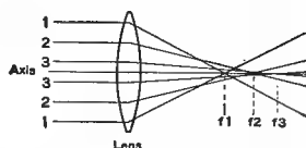
FIG. 168. SPHERICAL ABERRATION IN LENSES.
