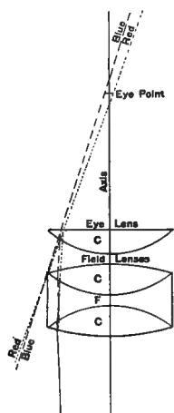
FIG. 174. POSITIVE COMPENSATION OCULAR. (From Spitta, p. 110).
