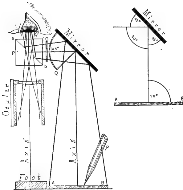
FIG. 100. DIAGRAM OF ABBE'S CAMERA LUCIDA WITH A VERTICAL MICROSCOPE.
