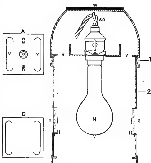
FIG. 37. LANTERN FOR DAYLIGHT GLASS IN SECTION \times \frac{1}{4} .
