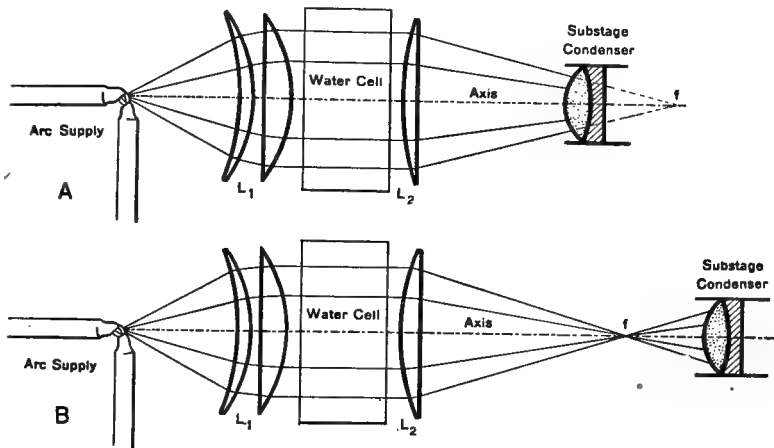
FIG. 115. DIAGRAMS TO SHOW THE POSITION OF THE SUBSTAGE CONDENSER WHEN NO PARALLELIZING LENS IS USED.
