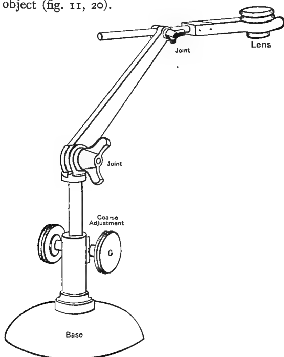
FIG. 19. ADJUSTABLE LENS HOLDER WITH JOINTS.
