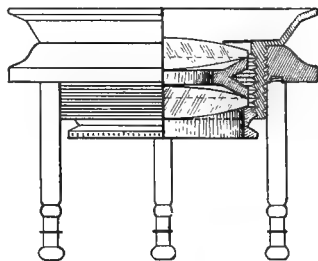
FIG. 18. TRIPOD MAGNIFIER WITH A SECTION REMOVED TO SHOW THE TWO COMPONENT, CONVEX LENSES AND INTERVENING DIAPHRAGM.
