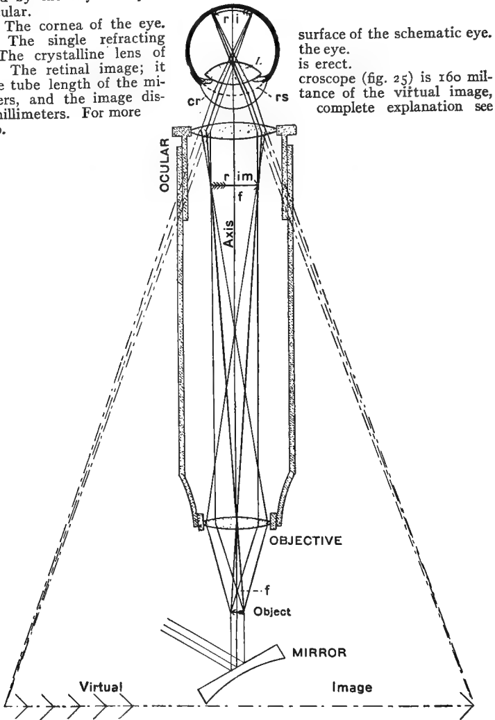
FIG. 78. COMPOUND MICROSCOPE SHOWING ALL THE IMAGES.
