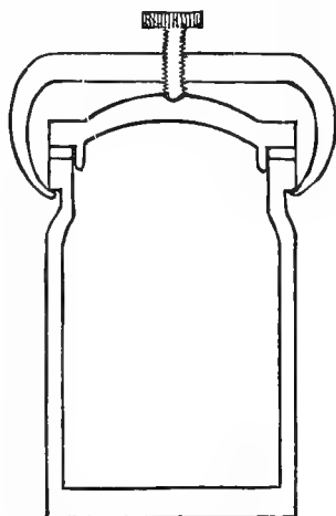
FIG. 214. SPECIMEN JAR WITH CLAMP.
