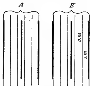
FIG. 90. THE IMAGES OF THE OCULAR AND OF THE STAGE MICROMETER, SHOWING HOW TO ARRANGE THE LINES.
