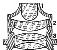
FIG. 138. ACHROMATIC SUBSTAGE CONDENSER FOR PHOTO-MICROGRAPHY.
