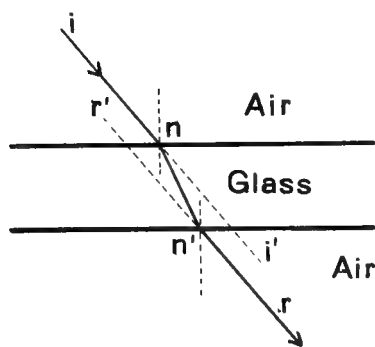
FIG. 157. DISPLACEMENT OF A RAY OF LIGHT IN TRAVERSING AN OBJECT WITH PLANE FACES.
