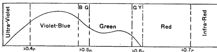
FIG. 141. NORMAL SPECTRUM SHOWING THE SENSITIVENESS OF ORTHOCHROMATIC OR ISOCHROMATIC PLATES.
