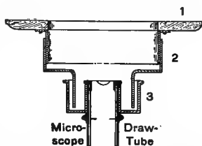
FIG. 134. LIGHT EXCLUDER FOR PHOTO-MICROGRAPHY.
