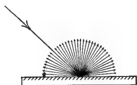
FIG. 153. IRREGULAR OR DIFFUSE REFLECTION.
