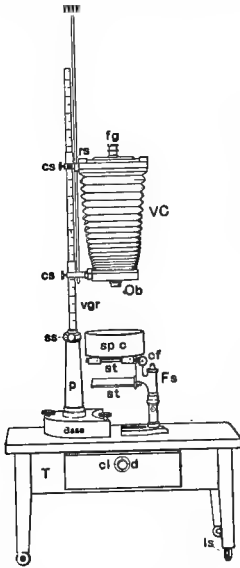
FIG. 126. VERTICAL PHOTOGRAPHIC CAMERA.
