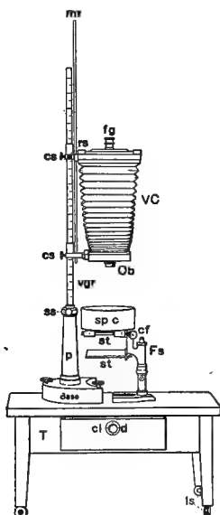
FIG. 107. VERTICAL PHOTOGRAPHIC CAMERA ON A LOW TABLE.
