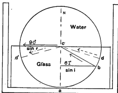
FIG. 160. CRITICAL ANGLE FOR LIGHT PASSING FROM GLASS TO WATER, THE ANGLE IN THE WATER BEING 90°.
