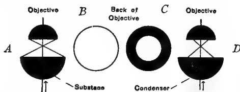
FIG. 45. APERTURE OF THE SUBSTAGE CONDENSER AND OF THE OBJECTIVE. (From Nelson, Jour. Roy. Micr. Soc.).
