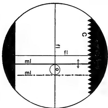
FIG. 94. FIELD OF THE MICROSCOPE SHOWING THE LINES AND THE RECORDING COMB OF THE FILAR MICROMETER (FIG. 93).
