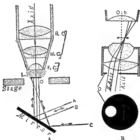
FIG. 67. OBLIQUE ILLUMINATION WITH A MIRROR AND WITH A CONDENSER.
