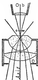
FIG. 42. SUB-STAGE CONDENSER WITH CONVERGING LIGHT.
