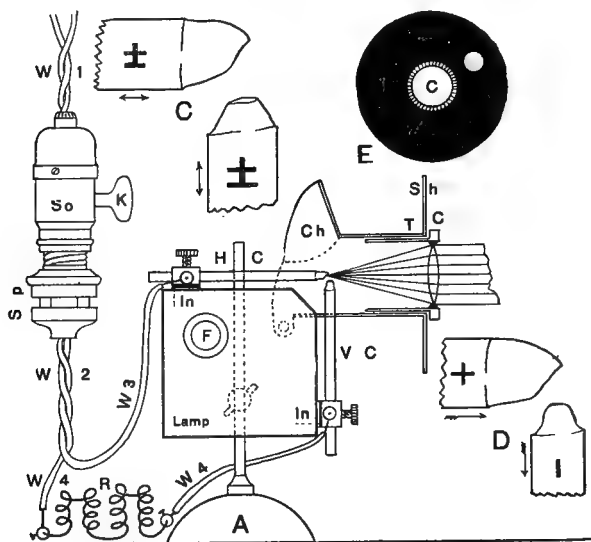
FIG. 49. SMALL ARC LAMP AND CONNECTIONS.
