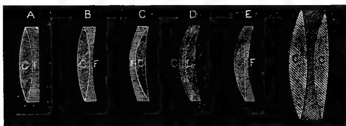
FIG. 173. ACHROMATIC COMBINATIONS OF CROWN AND FLINT GLASS LENSES. (From Lewis Wright's Optical Projection).
