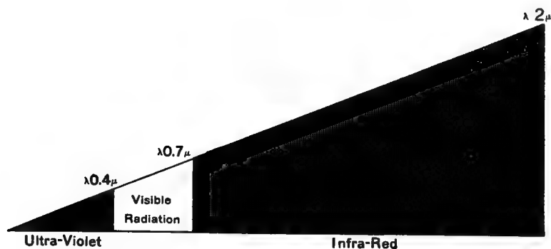
FIG. 151. VISIBLE AND INVISIBLE RADIATION.
