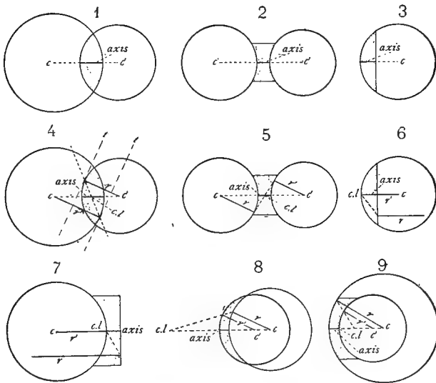
FIG. 167. SPHERICAL LENSES WITH THEIR FORMS AND PRINCIPAL FEATURES.
