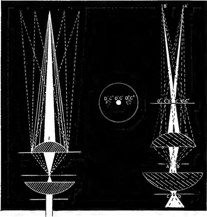
FIG. 178-179. DIFFRACTED LIGHT IN MICROSCOPY. (From Wright's Principles).
