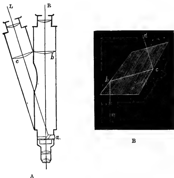
FIG. 52. WENHAM'S BINOCULAR MICROSCOPE.
