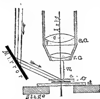
FIG. 34. LOW-POWER OBJECTIVE SHOWING WORKING DISTANCE AND REFLECTED LIGHT.
