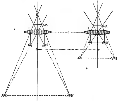
FIG. 87. DIAGRAM TO SHOW THAT THE SIZE OF THE VIRTUAL IMAGE OF A LENS DEPENDS UPON THE DISTANCE OF THE OBJECT FROM THE PRINCIPAL FOCUS.
