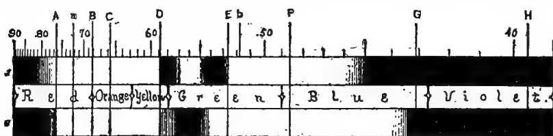
FIG. 149. ABSORPTION SPECTRUM OF ARTERIAL AND OF VENOUS BLOOD. (From Gamgee and McMunn).
