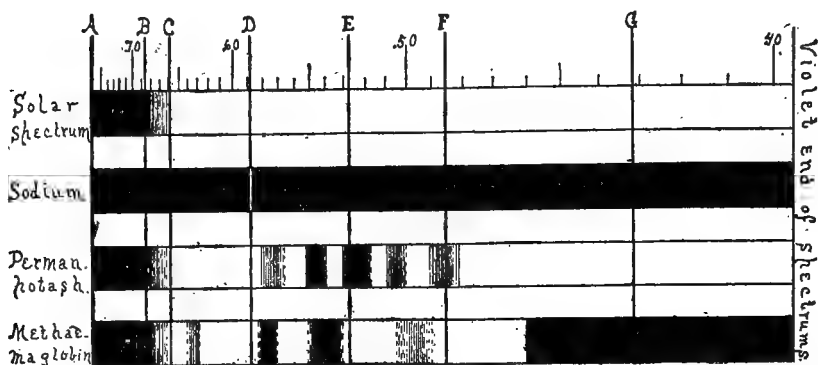
FIG. 148. SPECTRA TO SHOW DIFFERENT KINDS OF ABSORPTION BANDS.
