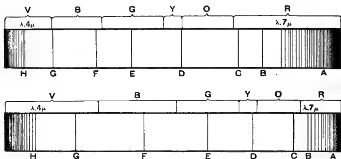
FIG. 146-147. A NORMAL AND A PRISMATIC SPECTRUM OF DAYLIGHT.
