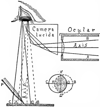
FIG. 99. WOLLASTON'S CAMERA LUCIDA.
