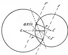
FIG. 8. LENS WITH OUTLINES OF THE TWO SPHERES OF WHICH IT IS SEGMENTS.
