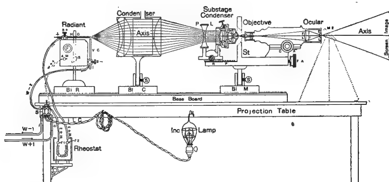
FIG. 131. HORIZONTAL PROJECTION MICROSCOPE FOR DRAWING AND FOR PHOTO-MICROGRAPHY.
