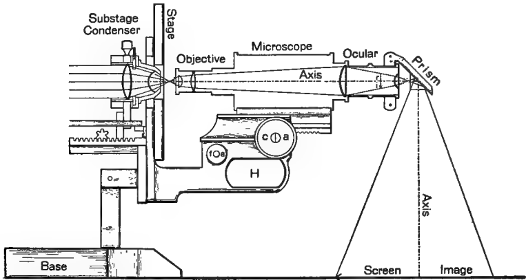
FIG. 114. THE MICROSCOPE ARRANGED FOR DRAWING ON A HORIZONTAL SURFACE.
