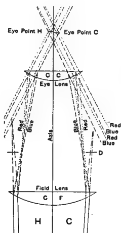
FIG. 175. HUYGENIAN OCULAR SHOWING THE ORDINARY AND THE COMPENSATING ACTION.
