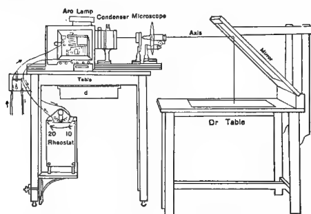
FIG. 246. DRAWING AND PROJECTION OUTFIT WITH LARGE MIRROR ON SEPARATE DRAWING TABLE.
