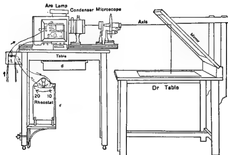
FIG. 112. PROJECTION MICROSCOPE WITH MOVABLE DRAWING TABLE AND 45° MIRROR.
