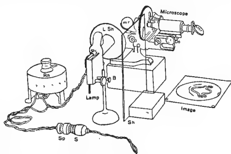
FIG. 113. DRAWING MICROSCOPE WITH SMALL ARC LAMP ON THE HOUSE LIGHTING SYSTEM.
