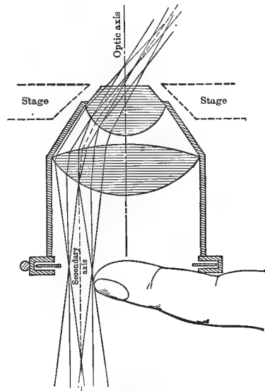
FIG. 46. OBLIQUE LIGHT WITH A CONDENSER.
