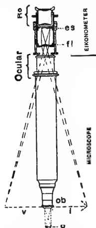
FIG. 96. WRIGHT'S EIKONOMETER.
