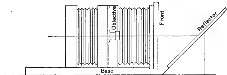
FIG. 108. CAMERA OBSCURA FOR DRAWING, AND LANTERN SLIDE MAKING. (From Optic Projection).
