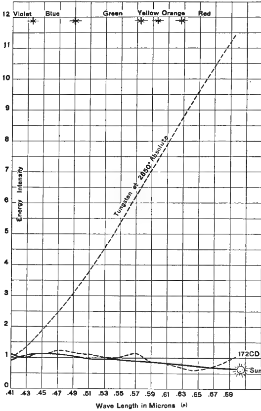
FIG. 36. CURVE OF ENERGY DISTRIBUTION IN MAZDA C LAMP, THE SUN AND THE LAMPLIGHT FILTERED THROUGH DAYLIGHT GLASS (172 CD).
