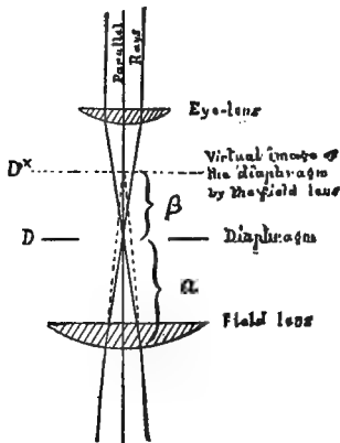
FIG. 184. PAR-FOCALIZATION OF OCULARS.
