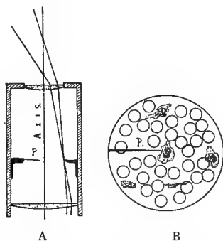
Fig. 117 A, B. POINTER OCULAR AND FIELD WITH POINTER.
