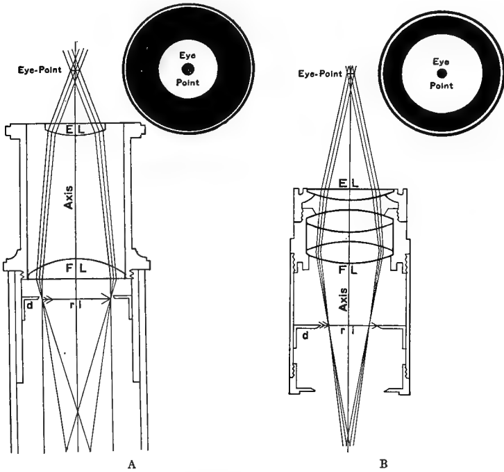
FIG. 22 A. RAMSDEN OCULAR WITH THE REAL IMAGE BELOW AND THE EYE-POINT ABOVE.
