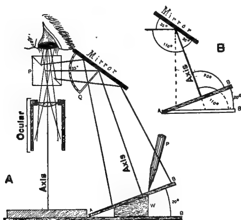
FIG. 101. DIAGRAM OF THE ABBE CAMERA LUCIDA WITH THE DRAWING SURFACE ELEVATED TO MAKE THE AXIS PERPENDICULAR WITH DEPRESSED MIRROR.
