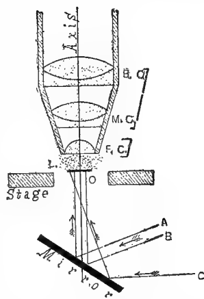
FIG. 35. HIGH-POWER IMMERSION OBJECTIVE WITH DIRECT AND OBLIQUE TRANSMITTED LIGHT.
