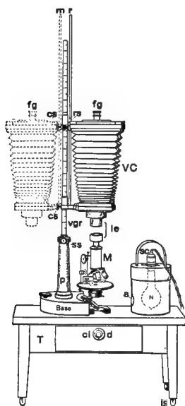
FIG. 129. VERTICAL MICROSCOPE AND CAMERA FOR PHOTO-MICROGRAPHY.
