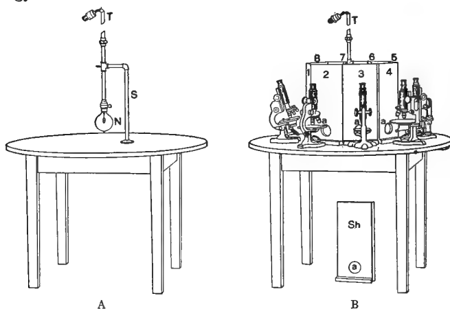
FIG. 124 A, B. KINGSBURY'S DEMONSTRATION TABLE WITH ARTIFICIAL DAYLIGHT. (ABOUT \frac{1}{25} NATURAL SIZE).
