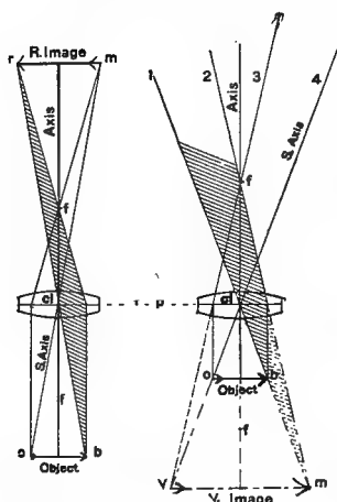
FIG. 163-164. TO SHOW THE FORMATION OF A REAL AND OF A VIRTUAL IMAGE BY A CONVEX LENS. (COMPARE FIG. 11-12).
