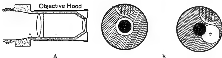
FIG. 123 A, B. METAL HOOD OVER THE OBJECTIVE TO AID IN CENTERING THE LIGHT.
