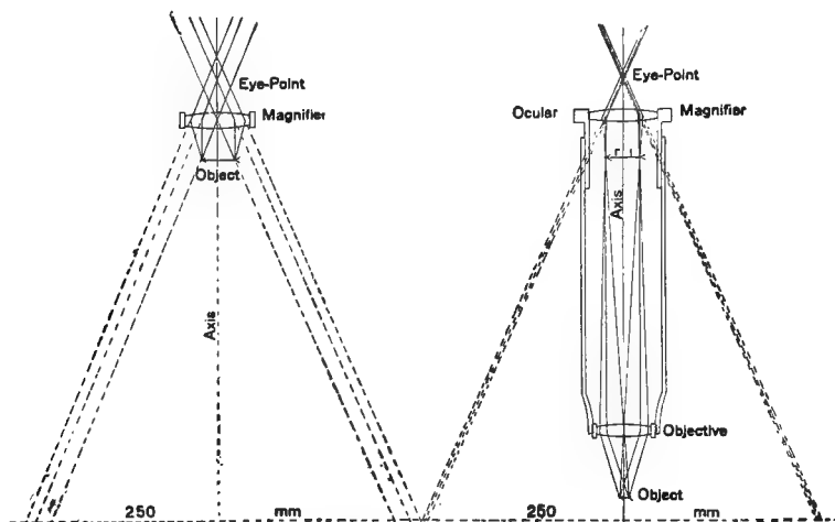
FIG. 88-89. DIAGRAMS OF SIMPLE AND COMPOUND MICROSCOPES WITH PARALLEL BEAMS EMERGING ABOVE AND PROJECTED BELOW.
