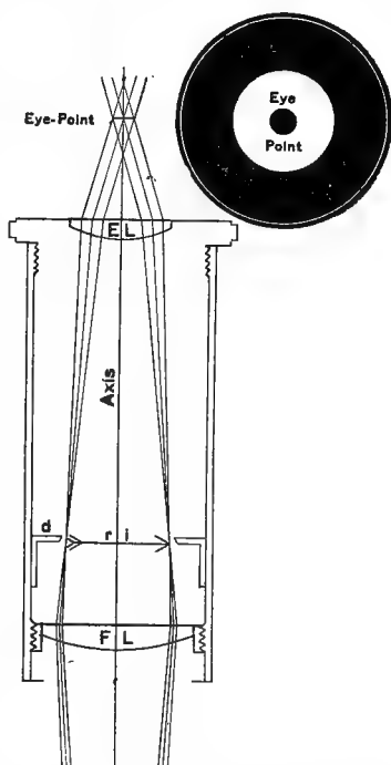
FIG. 23. LOW-POWER HUYGENIAN OCULAR IN SECTION.
