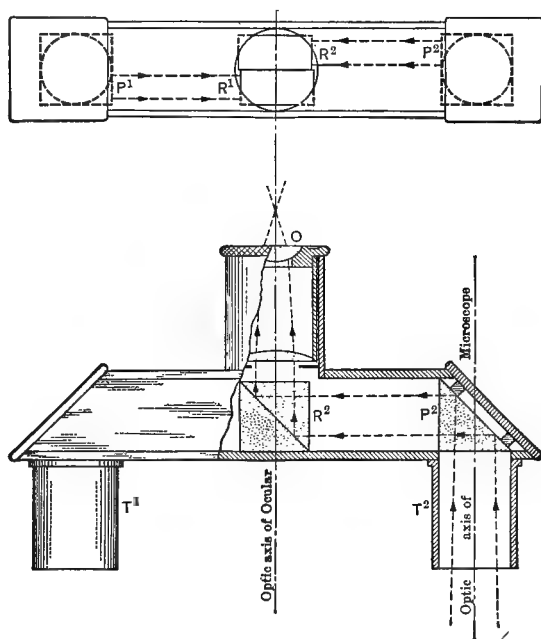
FIG. 74. COMPARISON OCULAR FOR PLACING HALF THE FIELDS OF TWO MICROSCOPES SIDE BY SIDE. ( R^1 R^2 ).
