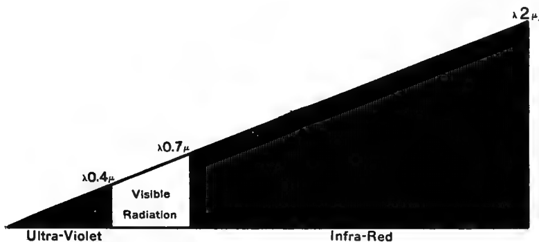
FIG. 144. NORMAL SPECTRUM SHOWING VISIBLE AND INVISIBLE RADIATION. (Magnified 20,000 times vertically and 50,000 times horizontally). (From Optic Projection).
