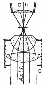
FIG. 41. SUBSTAGE CONDENSER OF ABBE WITH PARALLEL LIGHT.
