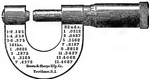
FIG. 188. MICROMETER CALIPERS FOR MEASURING THE THICKNESS OF SLIDES AND COVER-GLASSES.
