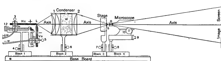
FIG. III. PROJECTION MICROSCOPE.
