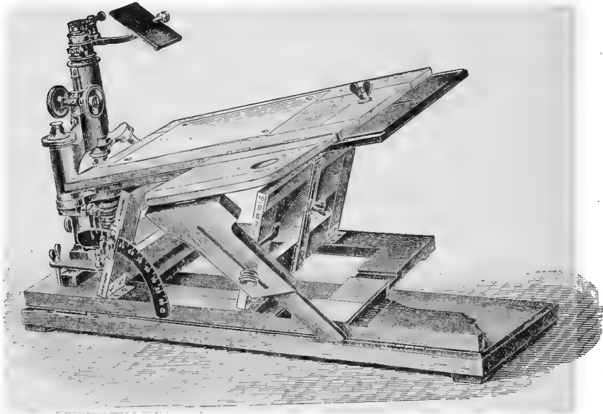
FIG. 102. BERNHARD'S DRAWING BOARD FOR THE ABBE CAMERA LUCIDA. (From the Catalogue of Zeiss).
