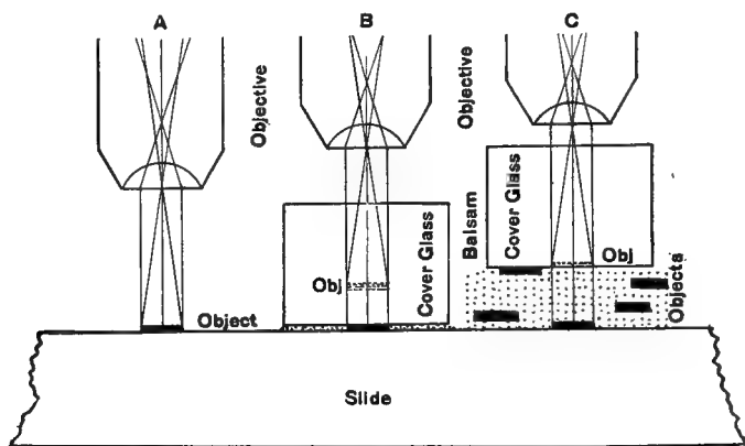
FIG. 30, 31, 32. WORKING DISTANCE AND THE COVER-GLASS.
