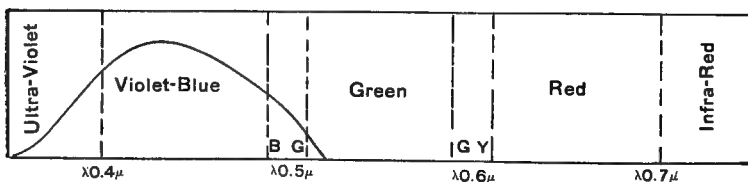
FIG. 140. NORMAL SPECTRUM SHOWING THE SENSITIVENESS OF ORDINARY PHOTOGRAPHIC PLATES.
