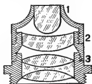
FIG. 39. ACHROMATIC SUBSTAGE CONDENSER.
