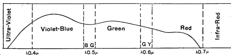
FIG. 142. NORMAL SPECTRUM SHOWING THE SENSITIVENESS OF PANCHROMATIC PLATES.
