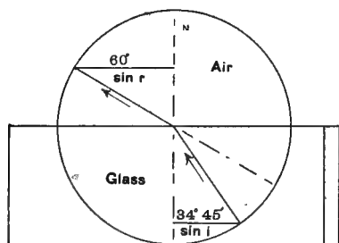
FIG. 156. REFRACTION OF LIGHT IN PASSING FROM GLASS TO AIR.
