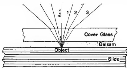
FIG. 51. ABERRATION PRODUCED BY THE COVER-GLASS.
