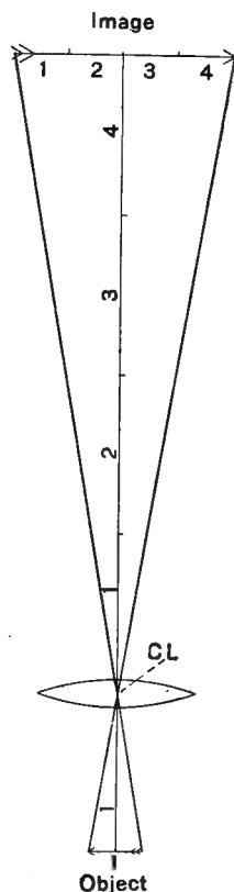
FIG. 84. TO SHOW THAT THE SIZE OF THE REAL IMAGE DEPENDS UPON ITS RELATIVE DISTANCE FROM THE CENTER OF THE OBJECTIVE.
