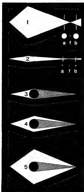
FIG. 180. EFFECT OF APERTURE ON DEFINITE FOCUS AND ON OVERCOMING OPACITIES.
