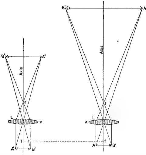
FIG. 86. DIAGRAMS TO SHOW THAT THE SIZE OF THE REAL IMAGE OF A LENS DEPENDS UPON THE DISTANCE OF THE OBJECT FROM THE PRINCIPAL FOCUS.
