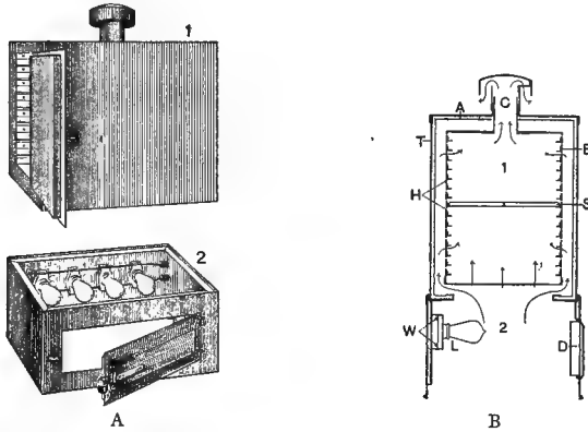
FIG. 244. DRYING OVEN FOR SLIDE TRAYS.
