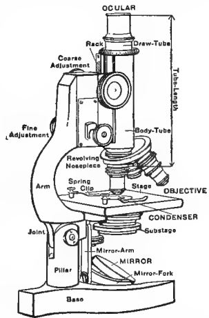
FIG. 170. THE MICROSCOPE SHOWING TUBE-LENGTH.
