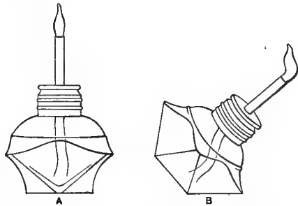
FIG. 227. ALCOHOL LAMP IN A VERTICAL AND AN INCLINED POSITION.
