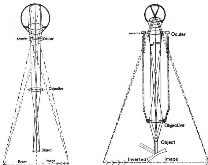
FIG. 248, 249. DUTCH AND KEPLERIAN COMPOUND MICROSCOPES FOR COMPARISON.
