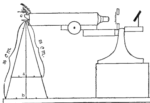
FIG. 85. DIAGRAM TO SHOW THAT THE SIZE OF THE VIRTUAL IMAGE DEPENDS UPON THE PROJECTION DISTANCE.
