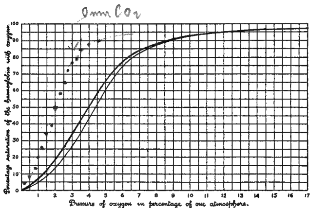
FIG. 1. Thick line—dissociation curve of oxyhaemoglobin in blood in the presence of 40 mm. pressure of CO 2 . Thin line—the dissociation curve of oxyhaemoglobin in blood within the body.
