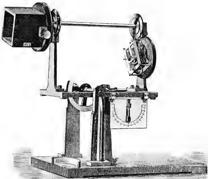
Klinostat with Adjustable Stand.
