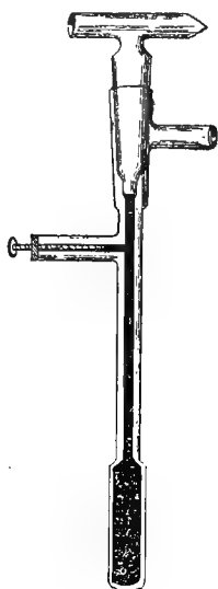
FIG. 23.—Reichert's Gas-regulator.
