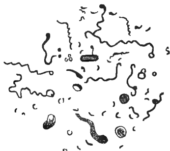
FIG. 101.—Involution forms of the spirillum of cholera.—( Van Ermengem. )
