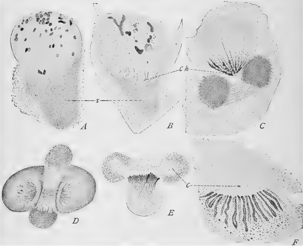
Fig. 70. — Nuclear division in Noctiluca miliaris .
