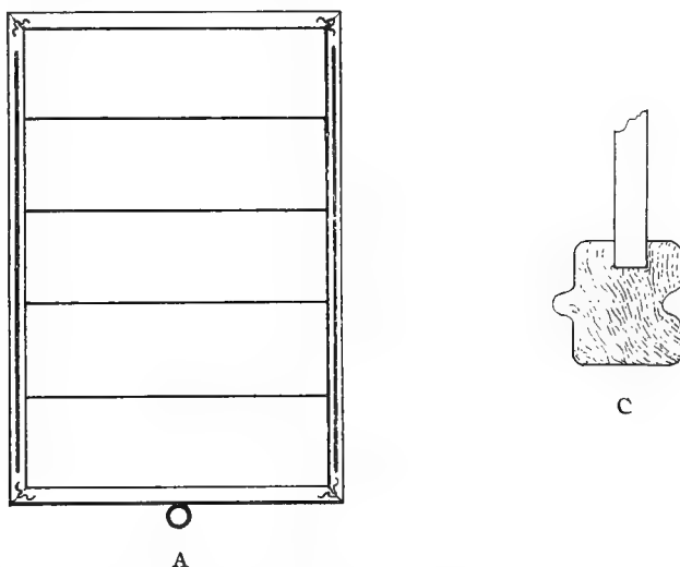
FIG. 213. Slide Tray with Cross Pieces on one Face to retain the Slides in Rows. (Dr. Greenman's improvement.) A tongue and groove serve to hold the trays in position when they are piled up. ( A , about 1-8, and C , about natural size.) The corners of the tray frame are held in place by the corrugated pieces of iron used in the construction of picture frames.
