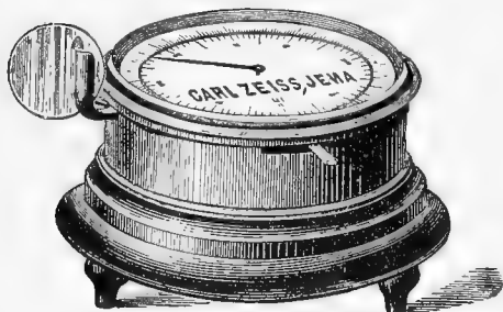
FIG. 196. Zeiss' Cover-Glass Measurer. With this the knife edge jaws are opened by means of a lever and the cover inserted. The thickness may then be read off on the face as the pointer indicates the thickness in hundredths millimeter in the outer circle and in thousandths inch on the inner circle.
