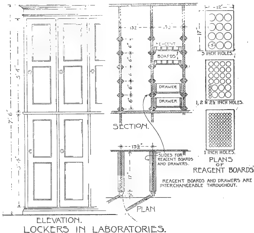
FIG. 214. Student Locker with trays and reagent boards. ( Jour. Appl. Micr. 1898, p. 127.)
