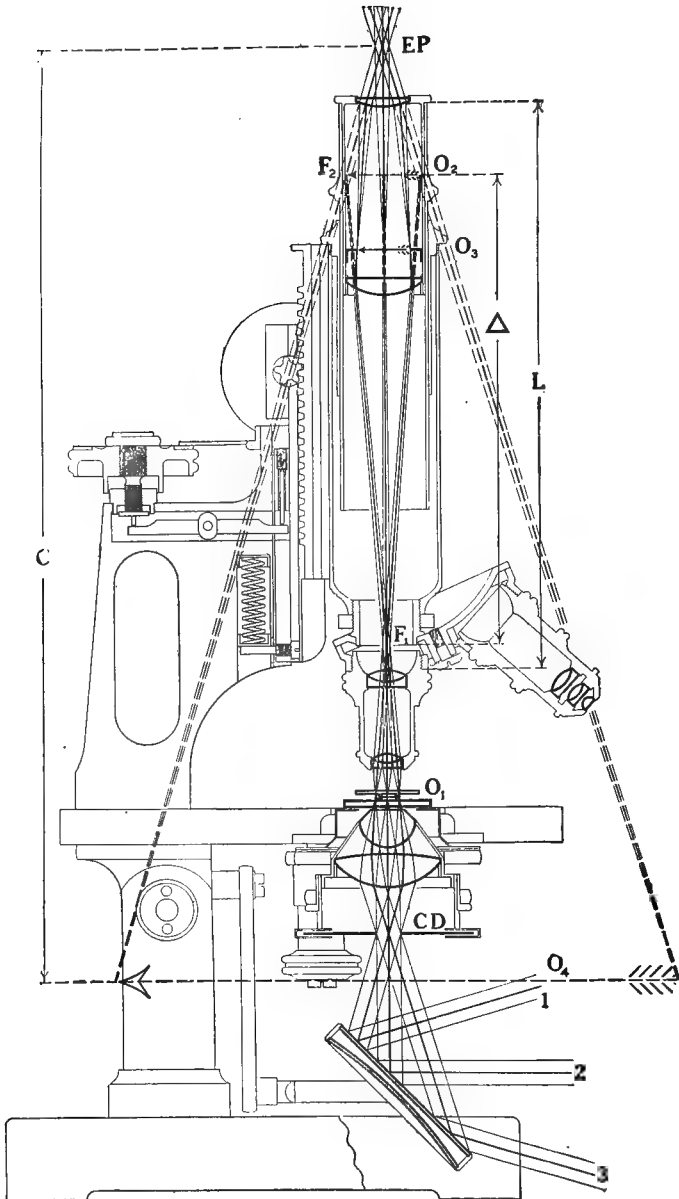
The Microscope in Section with the Images: 1, 2, 3, Beams of light to the mirror; C Image distance, i. e. : from eye-point, E-P, to virtual image ( O_4 ); CD Condenser diaphragm; EP Eye-point; F_1 Upper focal plane of the objective; F_2 Lower focal plane of the eye-piece; L Mechanical tube-length, i. e. : from top of draw-tube to screw for insertion of the objective; O_1 Object on the stage; O_2 Image formed by the objective were no field lens present; O_3 Image when field lens is present; O_4 Virtual image; \Delta Optical tube-length, i. e. : distance from the upper focal plane of the objective ( F_1 ) to lower focal plane of eye-piece F_2 .
