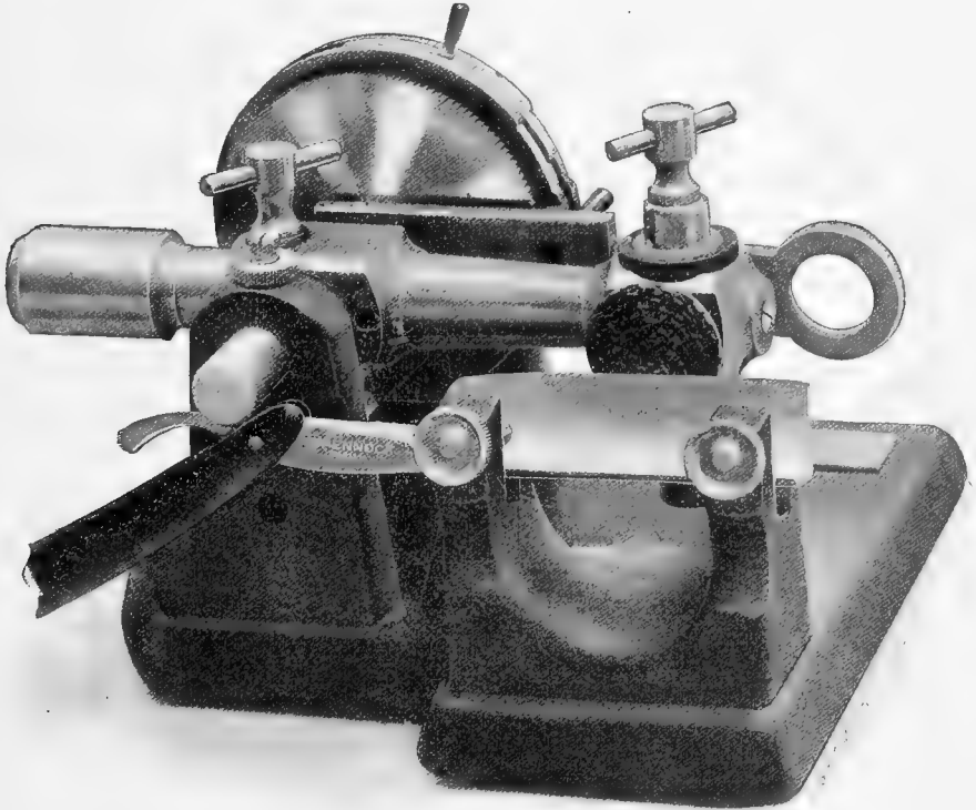
FIG. 235. The Conklin-Pietzsch automatic lever microlome for paraffin sectioning. This is a modified Ryder microlome and is simpler and therefore cheaper than most paraffin instruments. It is designed for sections from 1-300 to 10-300 mm. (3 1-3 to 33 1-3 \mu ). By means of a special attachment, sections of 2 \mu may be made. (Cut loaned by Edward Pennock, Philadelphia.)
