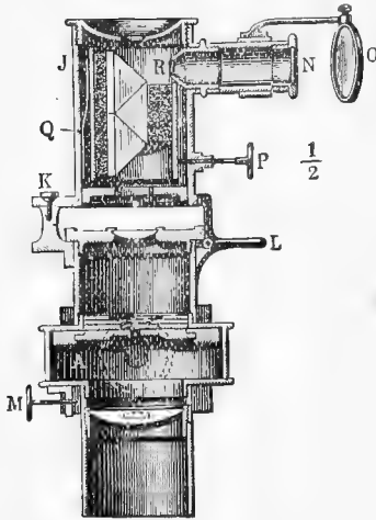
Abbe's Micro-spectroscope.
