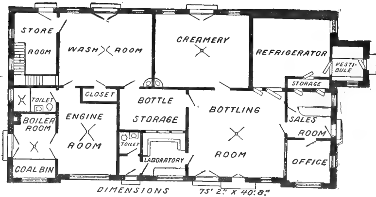
Floor plan of creamery and city milk plant.
