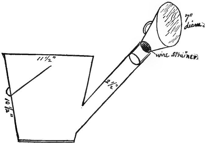
Modification of Stewart's Milk Pail.
