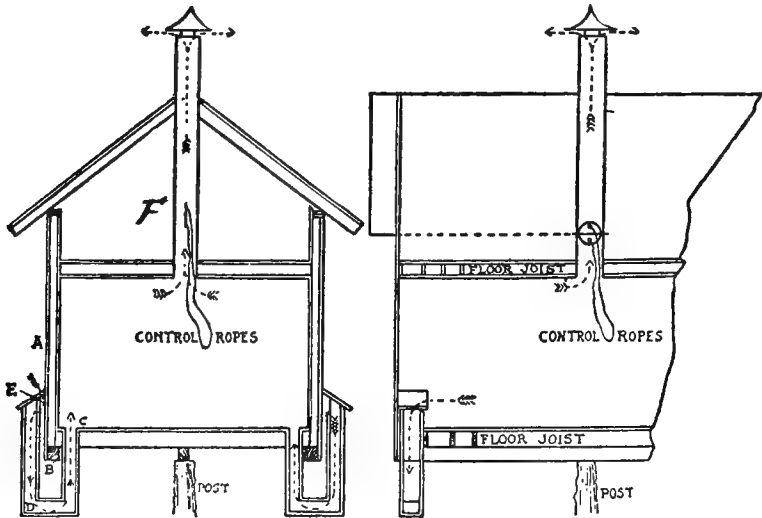
Sketch D—Showing the Rutherford System of Ventilation. (Hoard's Dairyman.)
