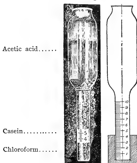
Tubes for Hart's Casein Test.
