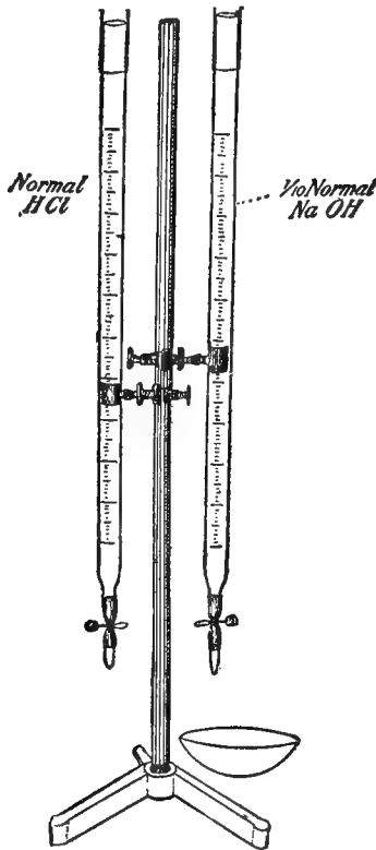
Two burettes arranged for titrating culture media.
