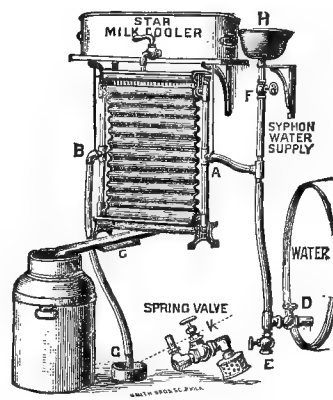
Star Milk Cooler.
