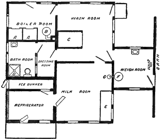
Floor plan of small plant for certified milk connected with barn. AA are coal bunkers; B , boiler; C , sterilizer; D , shower bath; E , bottling table; F , cooler; G , receiving can.
