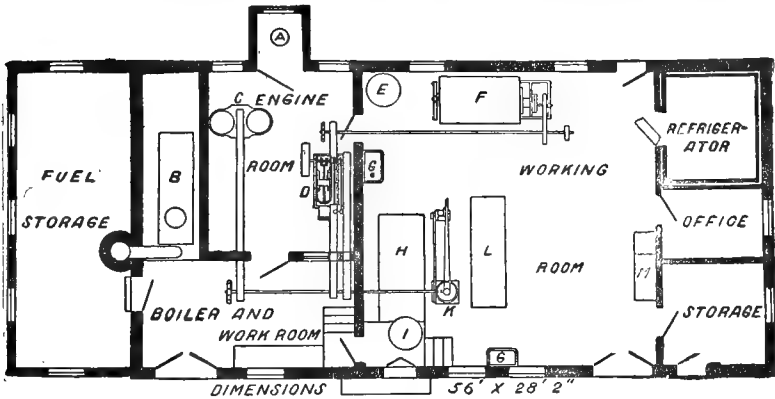
Floor plan of creamery for whole milk.
