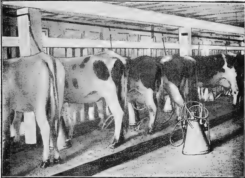
Fig. 98.—The Burrell-Lawrence-Kennedy Cow Milker.
