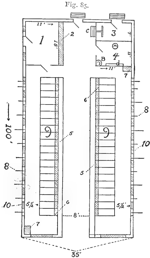
Rough Sketch of Ground Plan of Barn for Forty Cows, W. H. PAULHAMUS, Esq., Sumner, Washington.
