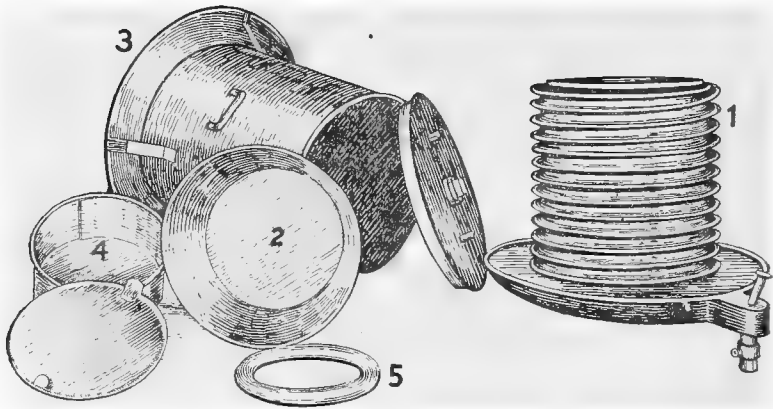
Parts of Cooler.
