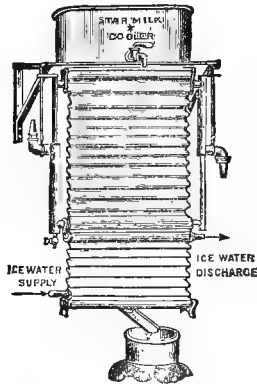
Star Milk Cooler.
