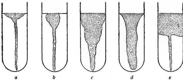
Types of Gelatin Liquefaction
