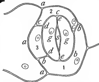
FIG. 629. — Stoma of Sedum ; a, u, u, first wall, cutting off mother cell of stoma; b, b, b, second; c, c, c, third; d, d, fourth; e, e, final wall; the latter, forming the two guard cells, g, g, partially splits to form the slit (s); 1, 2, 3, subsidiary cells.
