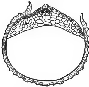
FIG. 308. — Female gametophyte of Selaginella : the apical cushion of cells having broken through the heavy megaspore wall; an archegonium to be observed at the apex. — After MISS LYON.
