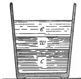
FIG. 623. — Diagram: c , chloroform; w , water; e , ether. that it separates determine the dominant direction of diffusion.
