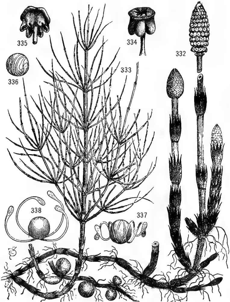
FIGS. 332-338. — Equisetum arvense : 332, fertile branches from the dorsiventral stem, each bearing a terminal strobilus, one of them mature; 333, sterile branch; 334, 335, two views of a sporangiophore (so-called "sporophyll"); 336-338, spores, showing the unwinding of the perinium. — After WOSSIDLO.
