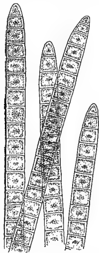
FIG. 6.— Oscillatoria : the cells of the simple filaments show the differentiation of the protoplast into the peripheral pigment region and the central region; in the center of the latter there appears an irregular aggregation of dark material ( chromatin ) characteristic of a nucleus.
