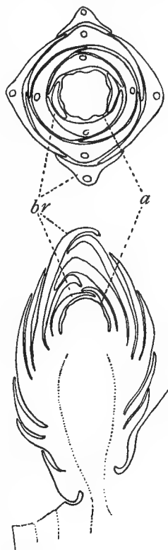
FIG. 473.—Cross and longitudinal sections of young staminate strobilus of Torreya , showing the overlapping bracts ( br ) and the position of the developing stamens ( a ).—After COULTER and LAND.
