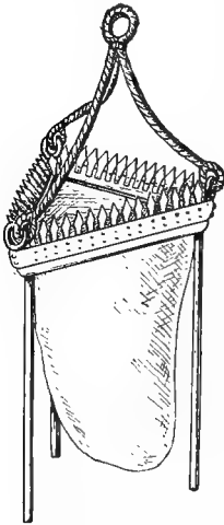
FIG. 1.—Reinke's Dredge.
