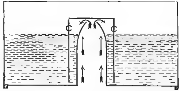
Sectional View of Fast Feeder.
