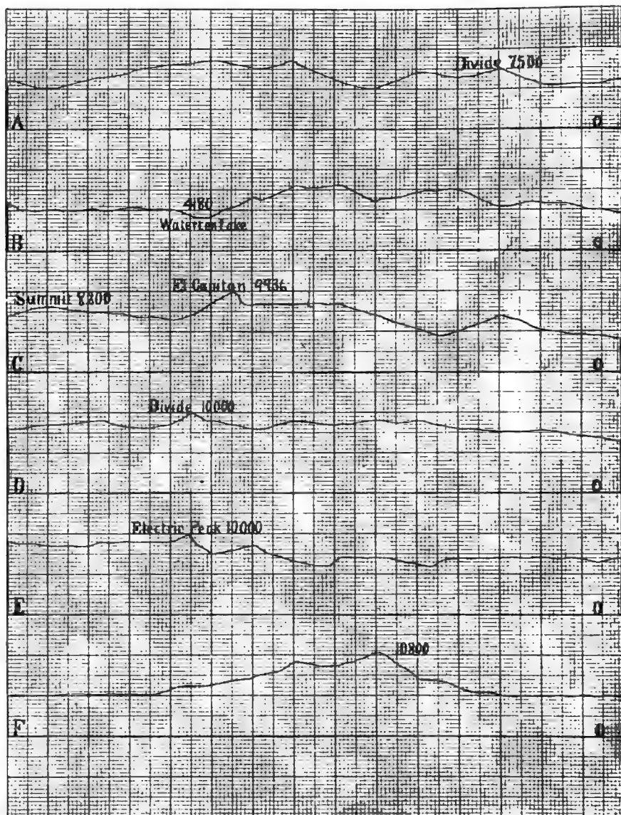
Fig. 5. Profiles of certain mountain ranges in Montana. Scale: horizontal and vertical, \frac{1}{2} inch: about 5000 feet. O, mean sea level. A and B, along the international border (49th parallel) from Kintla Lakes to Belly River, across Glacier National Park and the Continental Divide. C, section of the Bitter Root Range on the 46th parallel: from the summit to the Bitter Root River. D, Continental Divide on the 46th parallel. E, the Absaroka Range and the Yellowstone River on the 46th parallel. F, the Crazy Mountains on the 46th parallel.
