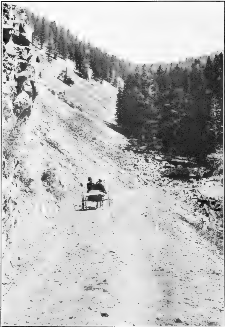
Fig. 36. A slide-rock slope, southern exposure, bearing Pinus ponderosa and Douglas spruce. Heavier forest to right Abies lasiocarpa , spruce and lodgepole pine. Near head of Bitter Root Valley, about 6000 feet, August.
