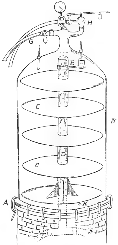
Fig. 18—BLACK FOREST STERILIZER.
