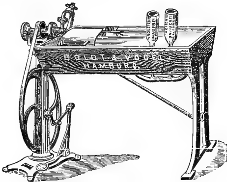
Fig. 27—COMBINED BRUSH AND RINSER.
