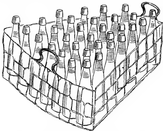
Fig. 19—MILK BOTTLES IN CARRIER READY FOR STERILIZING.
