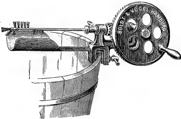
Fig. 25—CLEANSING BRUSH.
