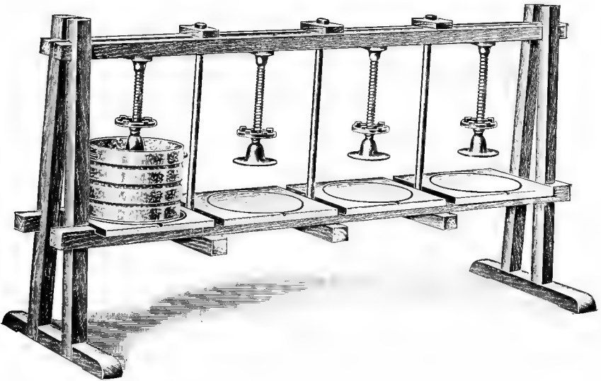
Upright Factory and Dairy Cheese Press
