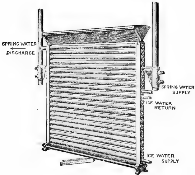
Fig. 6.—Tubular Cooler.
