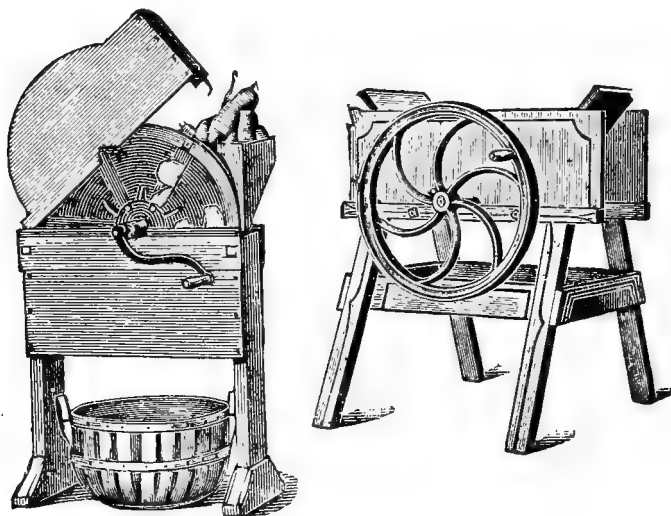
FIGS 36—37: ROOT CUTTERS
