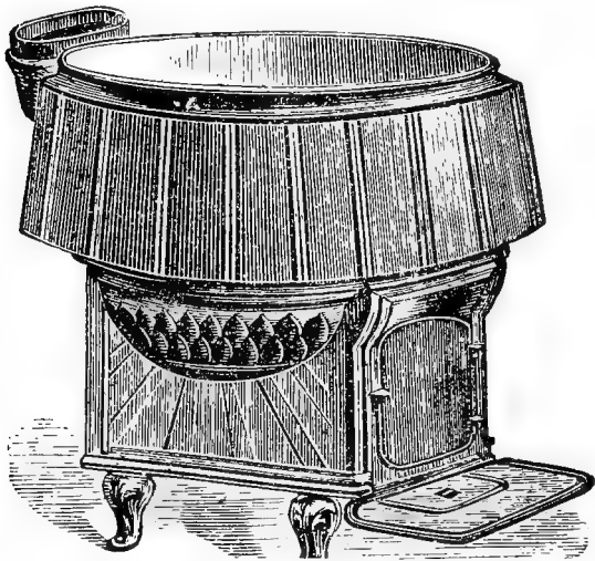
FIG 107: FEED COOKER
