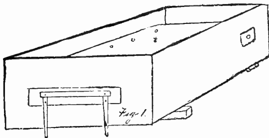
FIG 70: PLAN FOR HOMEMADE INCUBATOR
