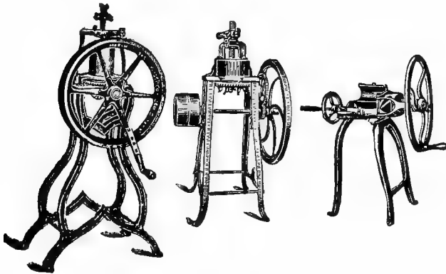
FIG 34: MOUNTED BONE MILLS
