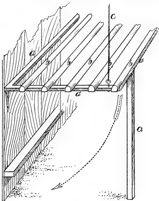
FIG 42: IMPROVED ROOST
