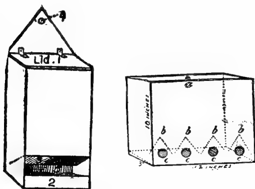
FIGS 8—9: AUTOMATIC FEEDERS
