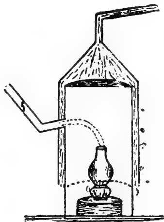
FIG 106: LAMP HEATER
