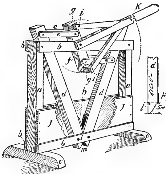
FIG 41: GRIT MILL
