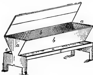
FIG 12: AUTOMATIC TROUGH
