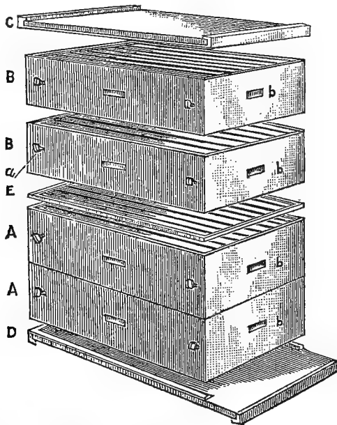
The Heddon Hive.—A, Bodies used as brood-chamber; B, Bodies used as super; C, Cover; D, Bottom board; Slated wood and zinc honey-board (Queen excluding); a, Wood thumb-screws; b, Handholes for lifting.
