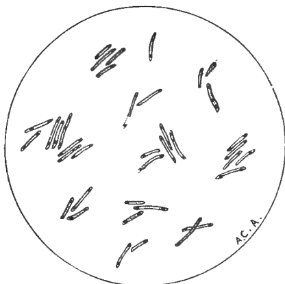
Bacillus diphtheriæ , stained by Neisser's method.
