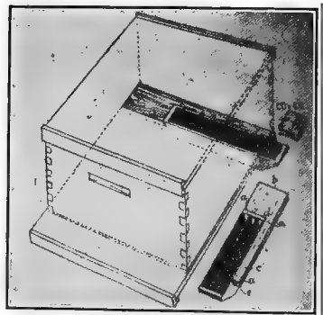
FIG. 28—THE ALEXANDER BOTTOM-BOARD FEEDER
