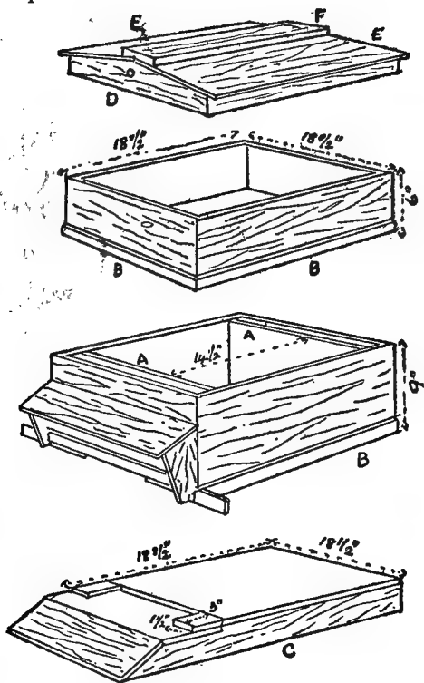
FIG. 7 Single-walled Hive
