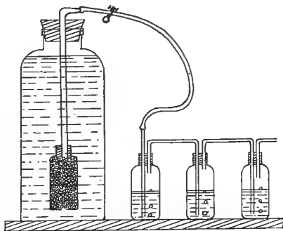
FIG. 32. Hydrogen Generator.
