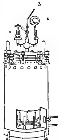
FIG. 4. Autoclave; a, safety valve; b, blow-off pipe; c, gauge; (Muir & Ritchie).
