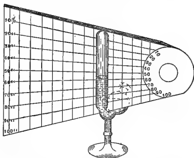
FIG. 19. Fermentation tube, showing method of using gasometer.
