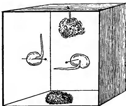
FIG. 3.—Germinating beans fixed on the sides of a box with a removable glass front. The beans are fixed with their roots pointing in different directions, but at the end of a few hours the tips of both roots will be seen to have curved round until they come to point vertically downwards.
