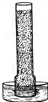
FIG. 18.—Experiment to demonstrate the rise of water in soils by capillary attraction.
