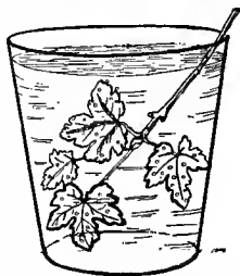
FIG. 13.— Experiment to show the bubbles of gas given off from leaves in sunlight.
