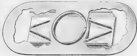
The Porter bee-escape, which is placed in the bee-escape board and traps the bees out of the supers.
