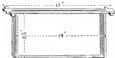
The Association Standard Frame, with Metal Ends.
