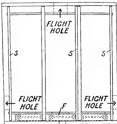
Fig. 24. Plan of Sladen's Nucleus Hive. s.s.s., Strips. f , Feeder in Wall.
